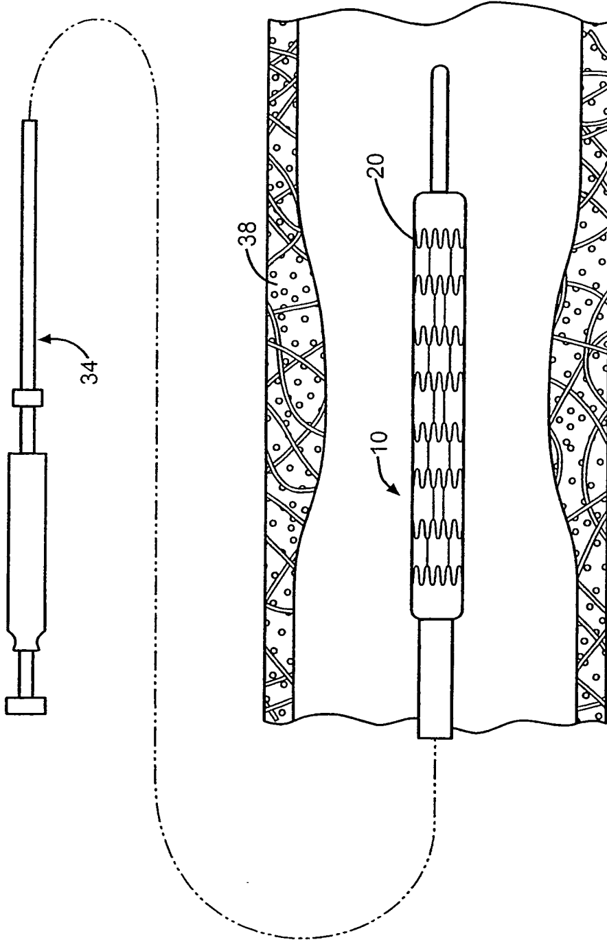
FIG. 1 (PRIOR ART)
