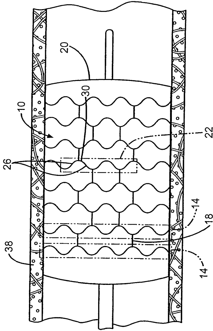
FIG. 2 (PRIOR ART)
