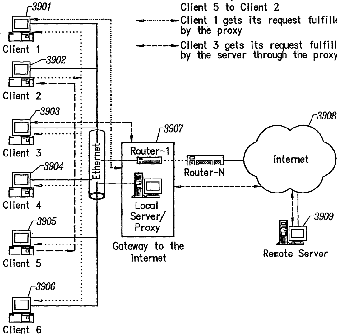
Client-Server System with Peer and Proxy Caching
