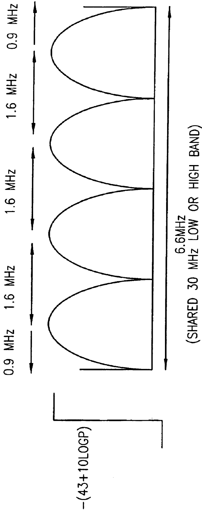
CONFIGURATION FOR 13.2 MHz TOTAL AVAILABLE BANDWIDTH
