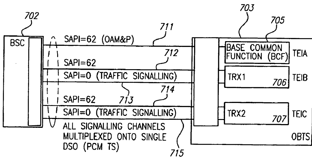
INTERFACE SIGNALLING STRUCTURES
