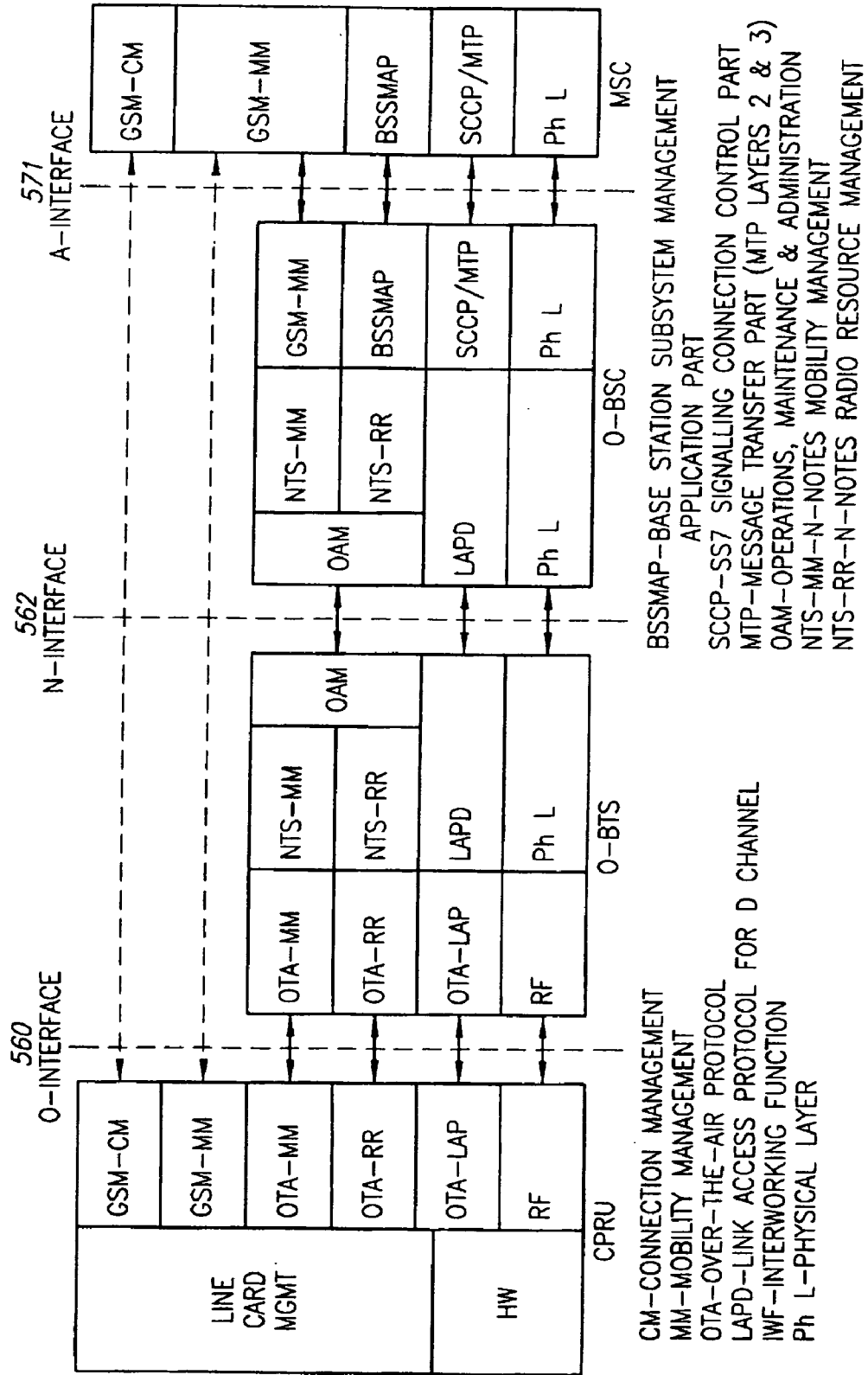
SYSTEM PROTOCOL ARCHITECTURE
