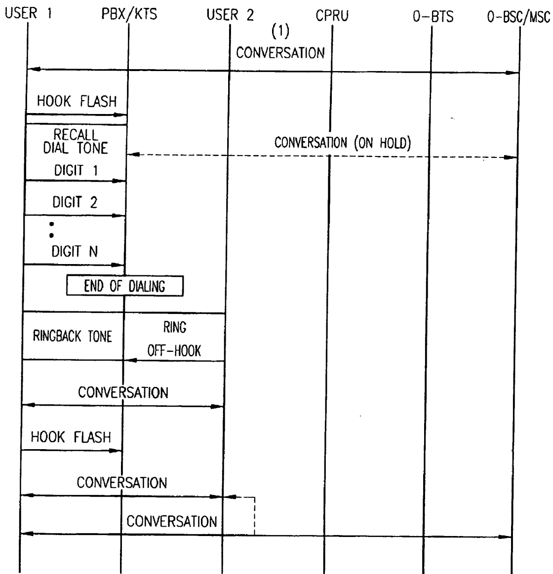
THREE-WAY CALL SETUP SCENARIO
