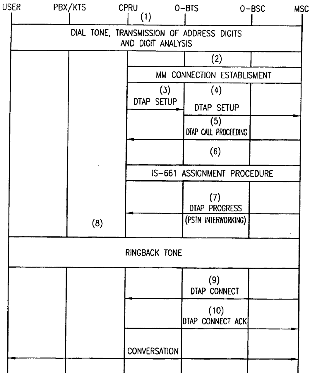
SUCCESSFUL OUTGOING CALL SETUP (PSTN INTERWORKING)
