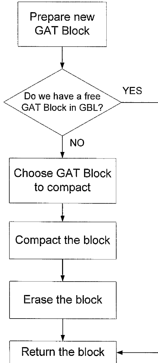
GAT Block Allocation
