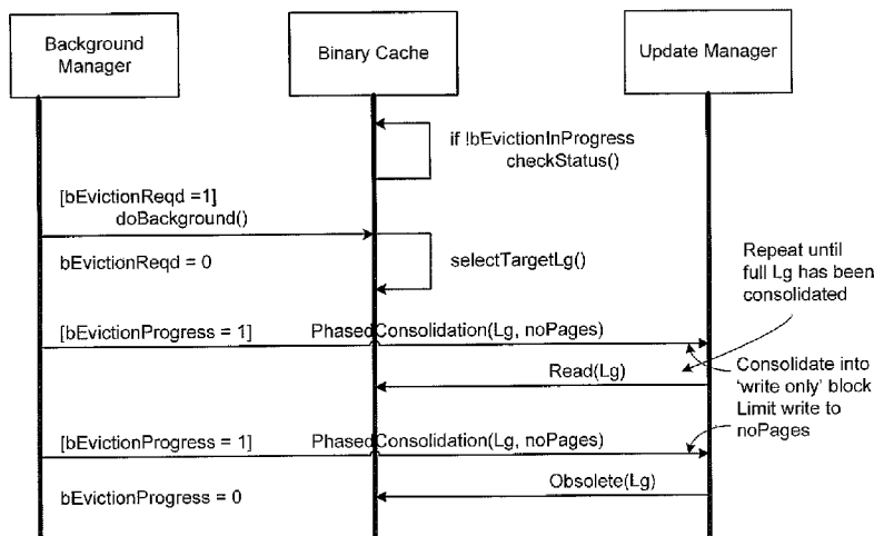
Binary Cache Eviction
