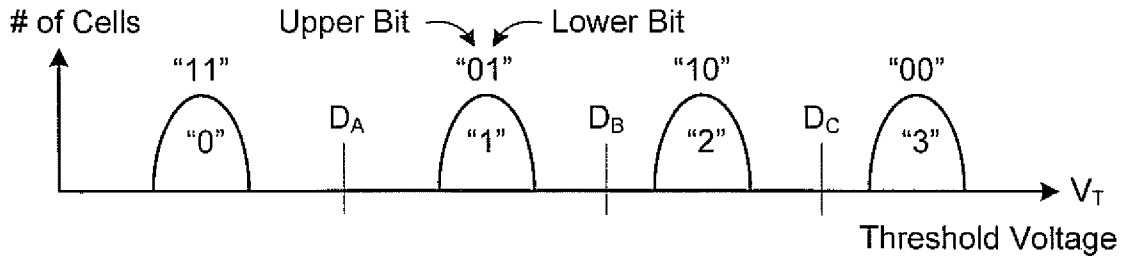
Multistate Memory
