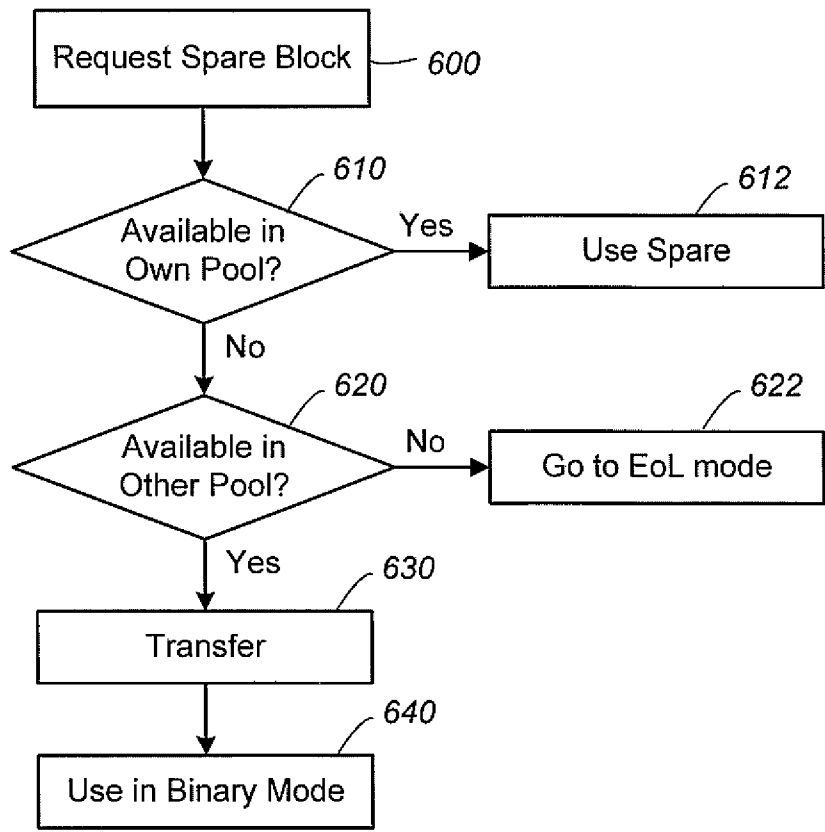
Spare Block Allocation from Main to BC
