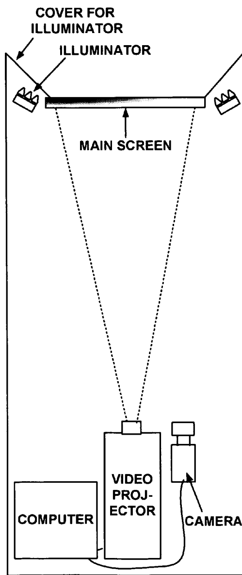
RECESSED DISPLAY SURFACE
