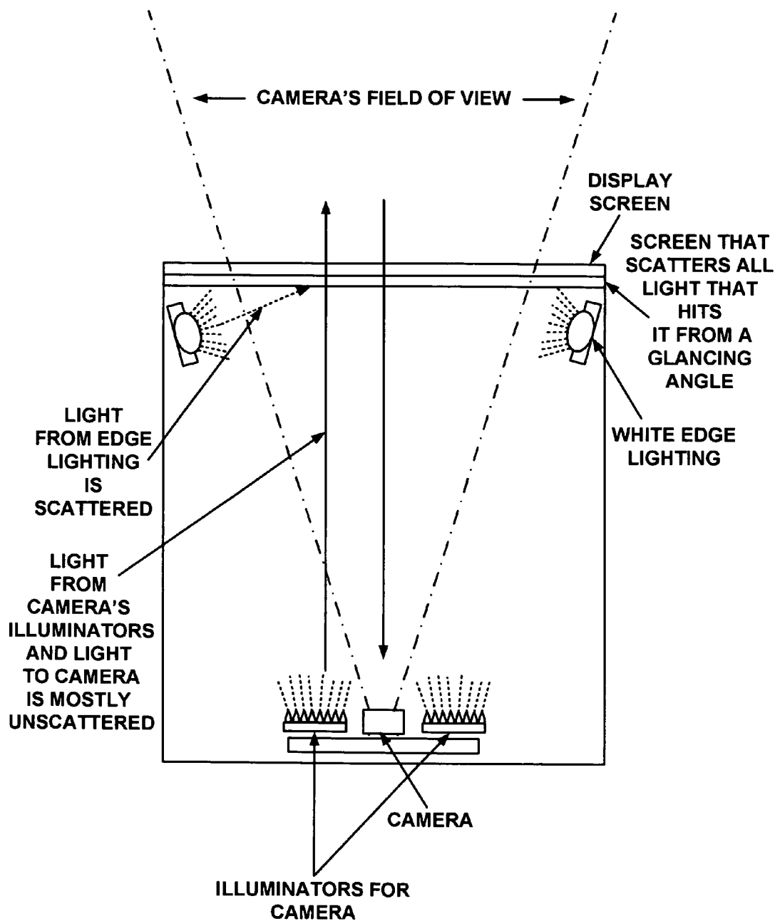
SAMPLE CONFIGURATION FOR EDGE LIGHTING
