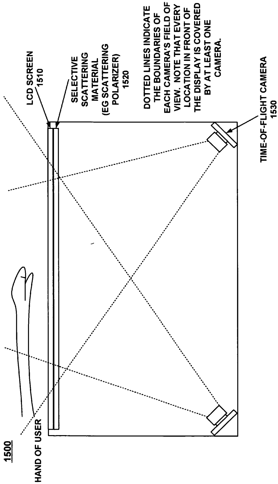
CAMERA/ILLUMINATION SUBSYSTEM FOR TIME-OF-FLIGHT CAMERAS
