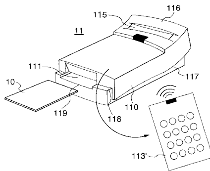
KEY ARRANGEMENT FOR IC CARD R/W
