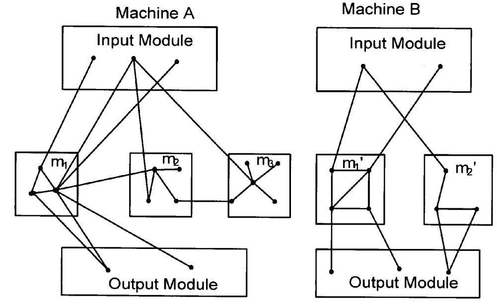
FIG. 4 CGE Crossover Before Crossover
