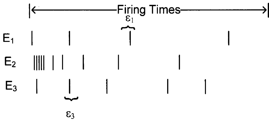
FIG. 5 Error Tolerance in Effectors
