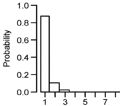
Unique tags per DRAM transfer for gcc
