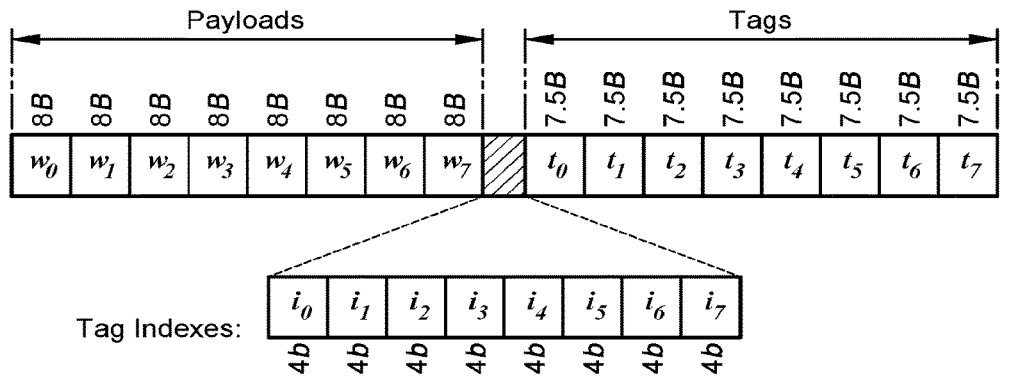
Cache line compression in DRAM
