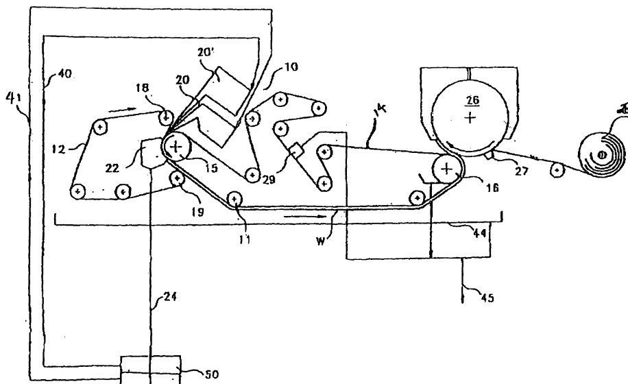
FIG. 1 -- CONVENTIONAL WET PRESS PROCESS LAYOUT
