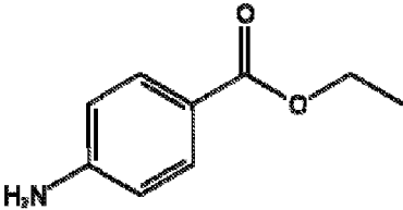
BENZOCAINE
