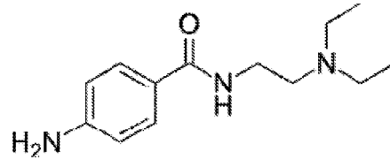
PROCAINAMIDE
