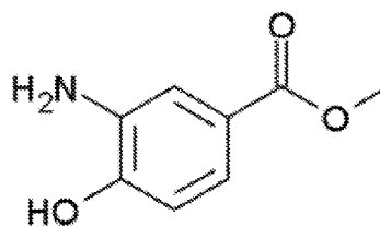
ORTHOCAINE
