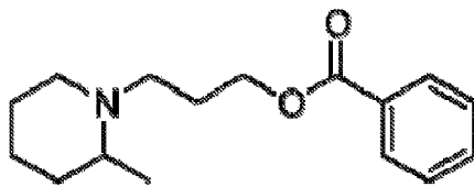
PIPEROCAINE
