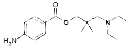
DIMETHOCAINE
