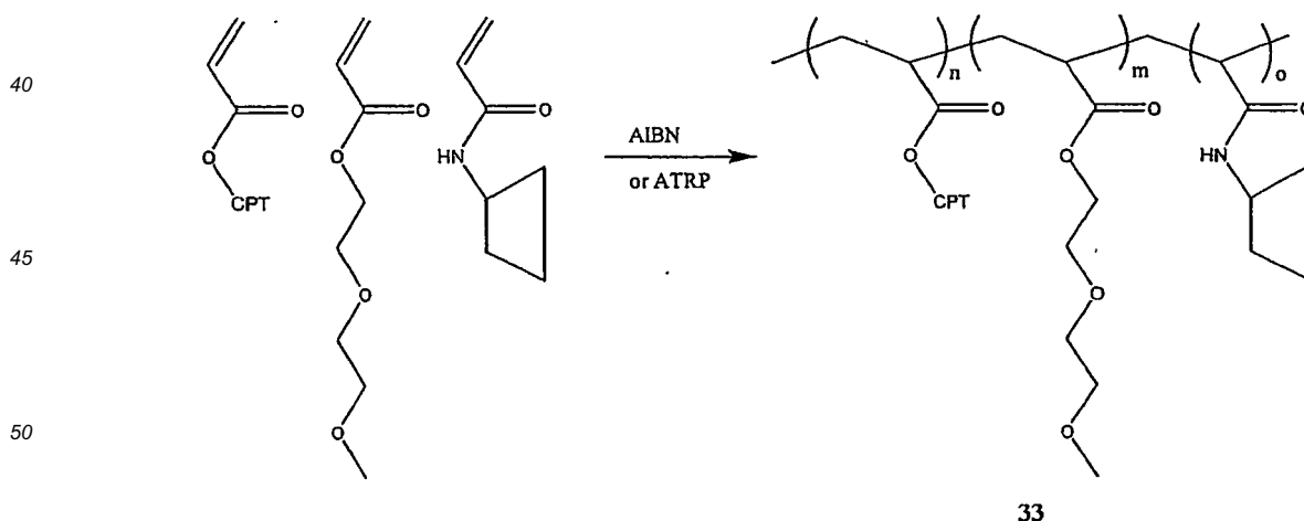
Scheme XXXV
