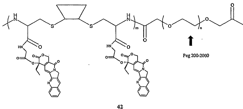
20 Scheme XXXXII
