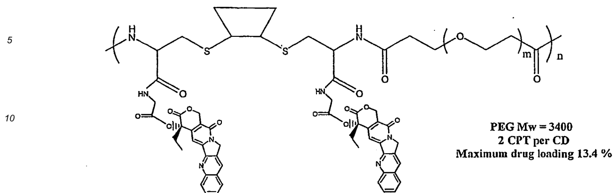
Scheme XXXXIII
