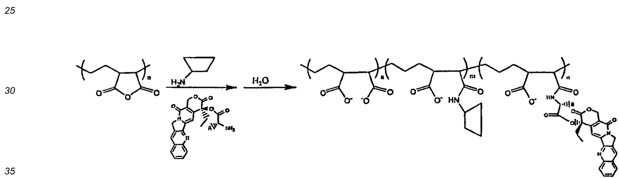
Scheme XI
