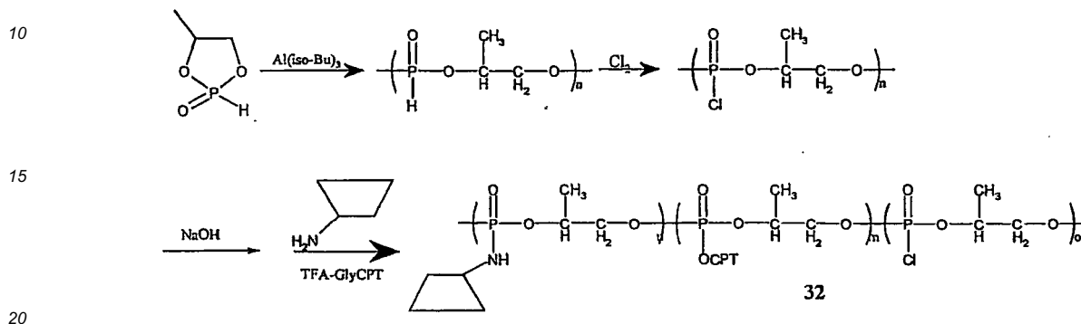
Scheme XXXIV
