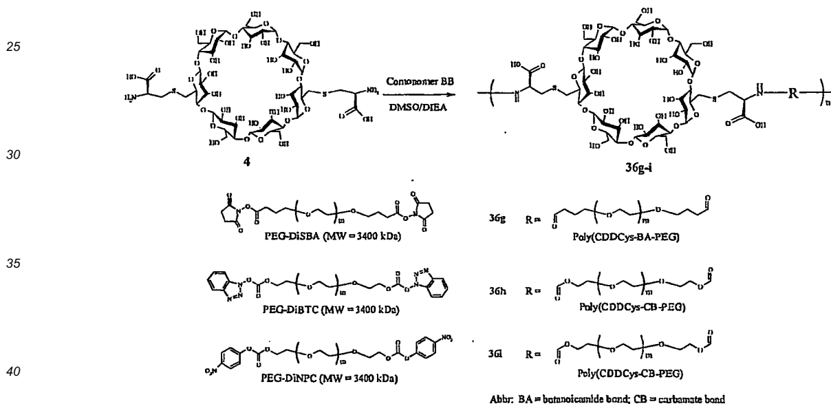
Scheme XXXVIIIb
