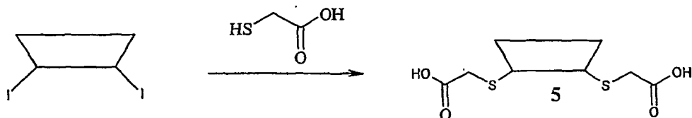
Scheme XIX
