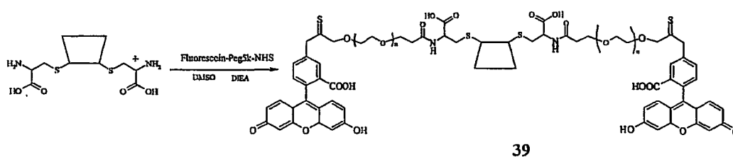
Scheme XXXX
