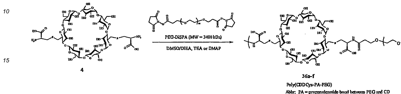
Scheme XXXVIIIa
