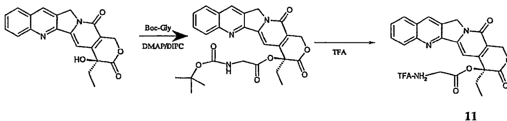
Scheme XXV
