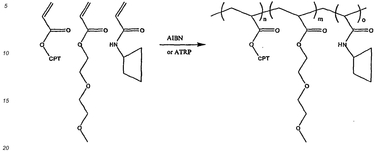
Scheme XI
