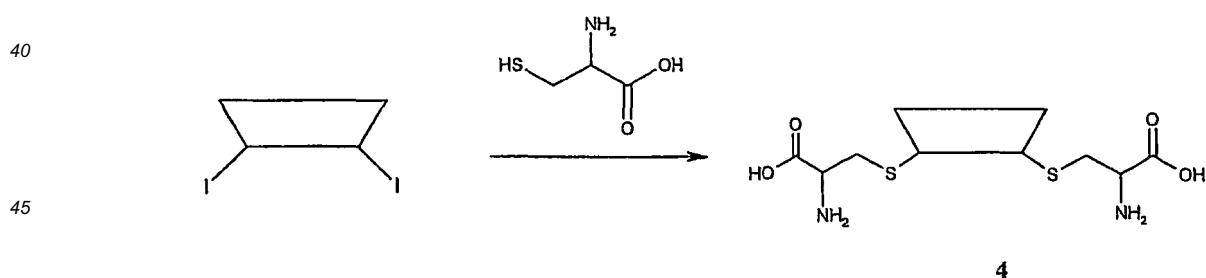
Scheme XVIII
