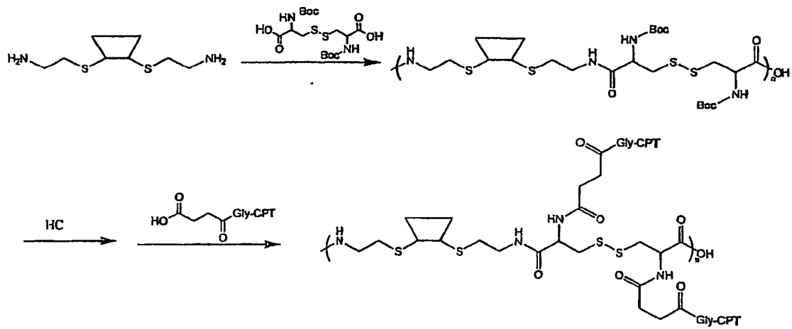
Scheme VII
