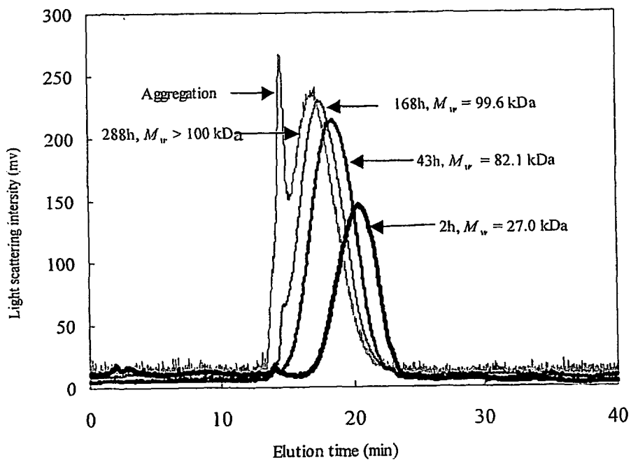
FIG. 5b: Polymerization control by adjusting polymerization time.
