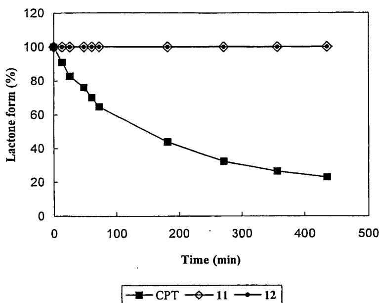
FIG. 3: Lactone Ring Stability of CPT, 11 and 12 in PBS (pH 7.4)
