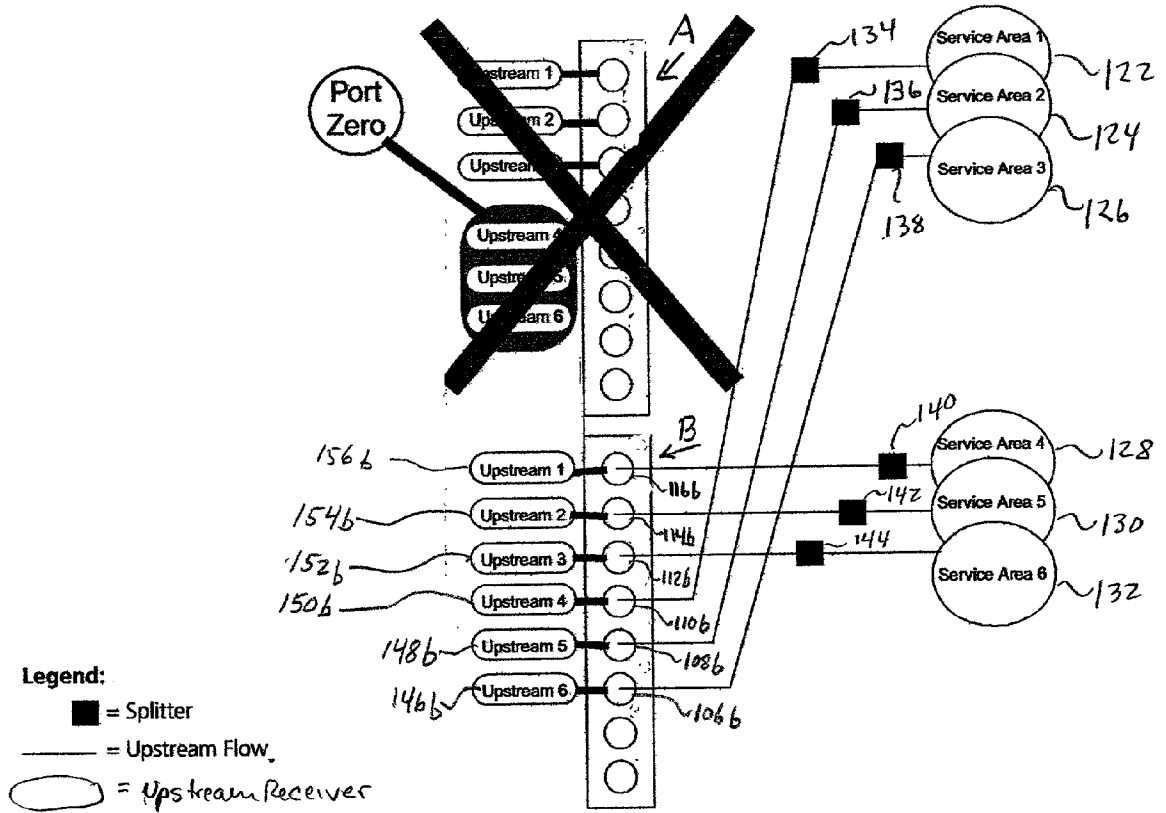
Sample Redundant Upstream Configuration (High Priority Data of VoIP, Failover)
