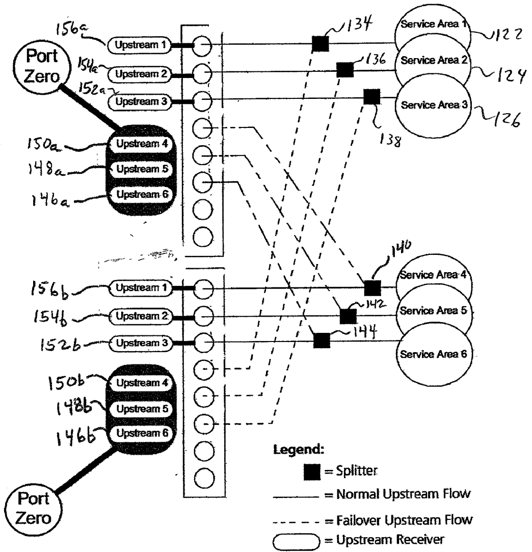
Sample Redundant Upstream Configuration (High Priority Data or VoIP, Normal)
