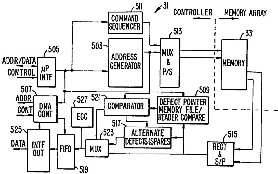
READ DATA PATH CONTROL
