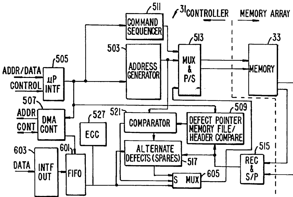
WRITE DATA PATH CONTROL
