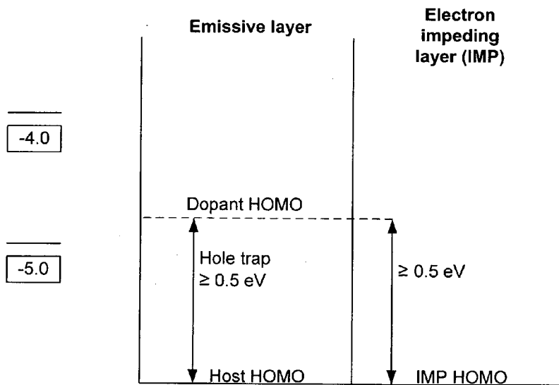
Figure 62: Exemplary HOMO Energy Levels for a Device Having an Electron Impeding Layer
