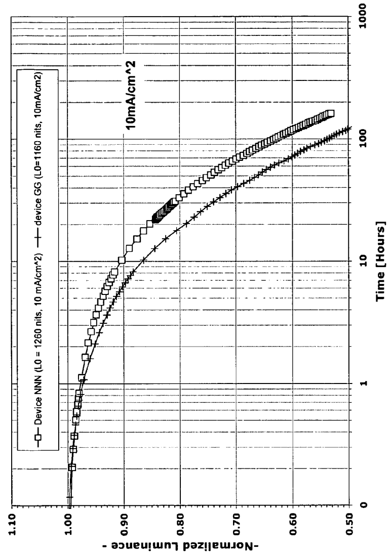
Figure 46 Lifetime – Devices GG and NNN
