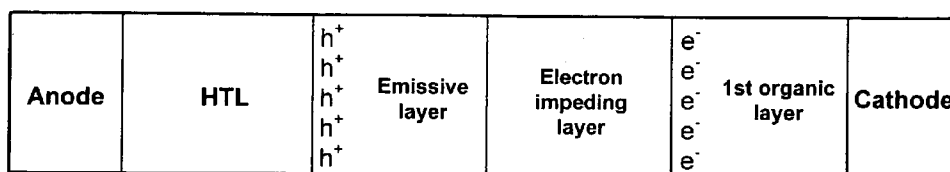
Figure 63a: Device Having an Electron Impeding Layer
