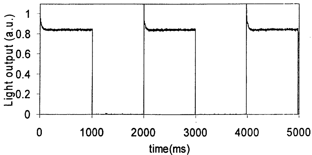
Figure 7: Light output for pulsed operation of OC 1 C 10 -PPV devices
