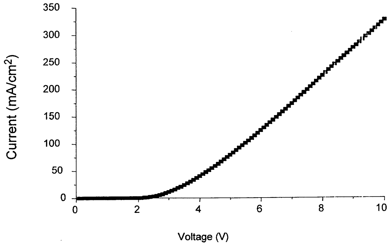
Figure 4(a): Current-voltage characteristics of device in figure 3
