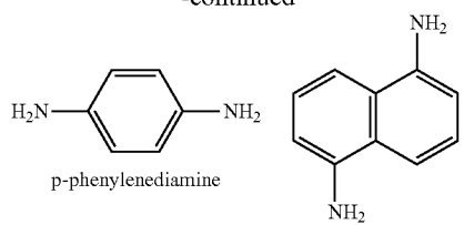
diaminonaphthalene
