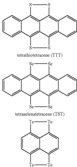
Formulae (D2): hetero cyclic donor containing sulfur
