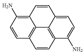
diaminopyrene
