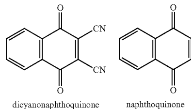
Formulae (A2): quinone type acceptor
