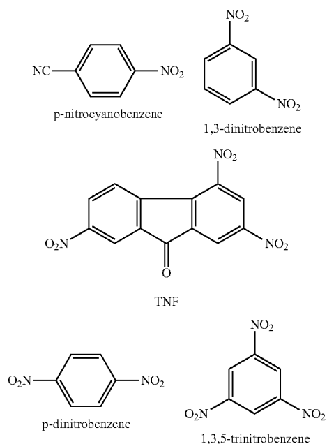
Formulae (A3): nitro compound type acceptor
