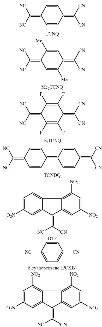
Formulae (A1): cyano type acceptor
