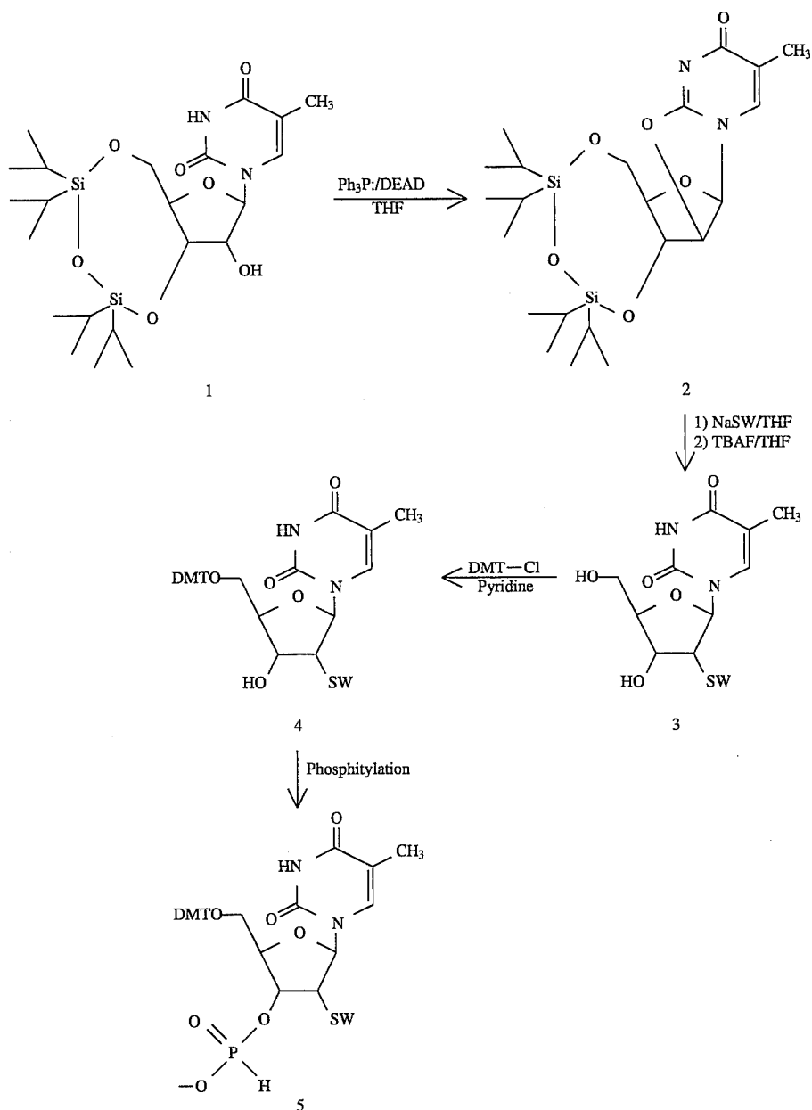
Reaction Scheme II
