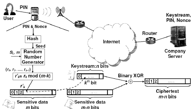
SE Scheme Working Flow Illustration.
