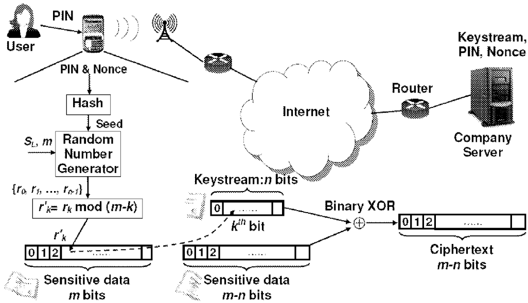
Figure 6. SE Scheme Working Flow Illustration.
