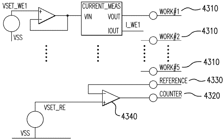
POTENTIOSTAT CONFIGURATION
