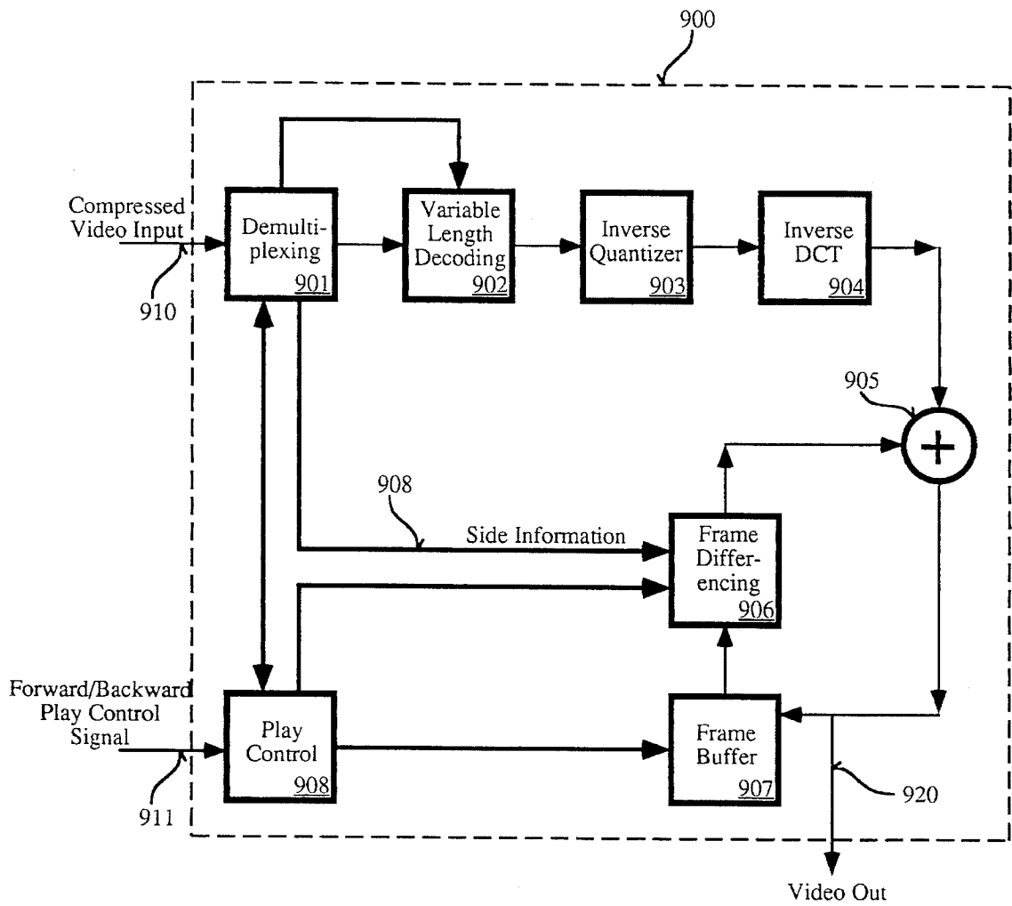
Figure 9 Enhanced CCITT Decoder
