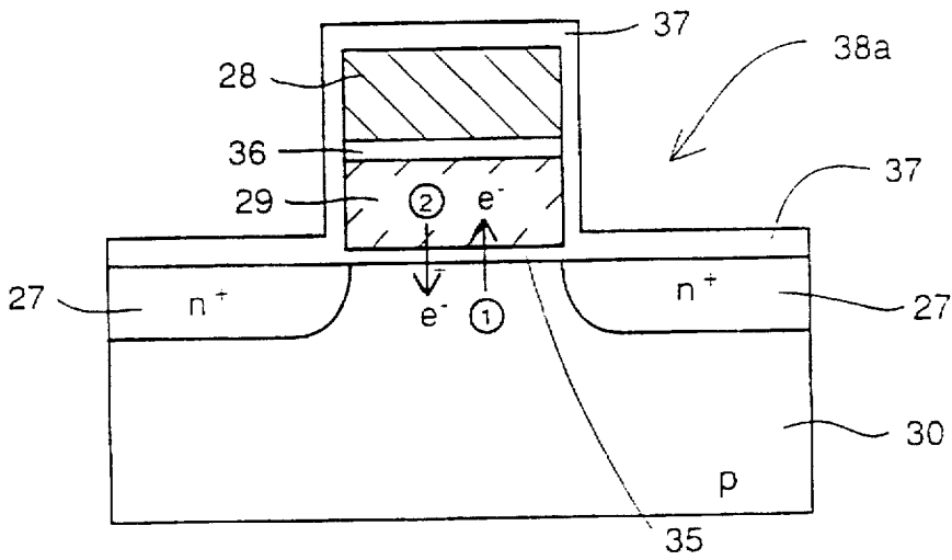
FIG. 155 PRIOR ART
