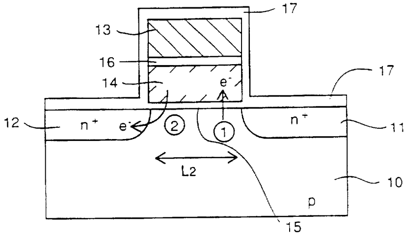
FIG. 151 PRIOR ART
