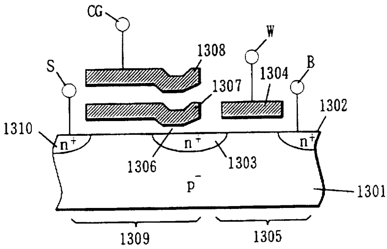
FIG. 143 PRIOR ART
