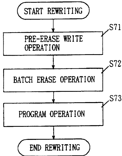
FIG. 141 PRIOR ART
