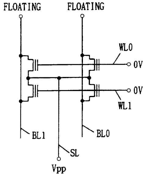
FIG. 136 PRIOR ART
