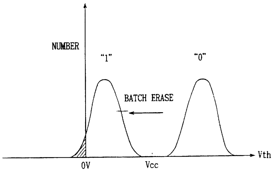
FIG. 142 PRIOR ART
