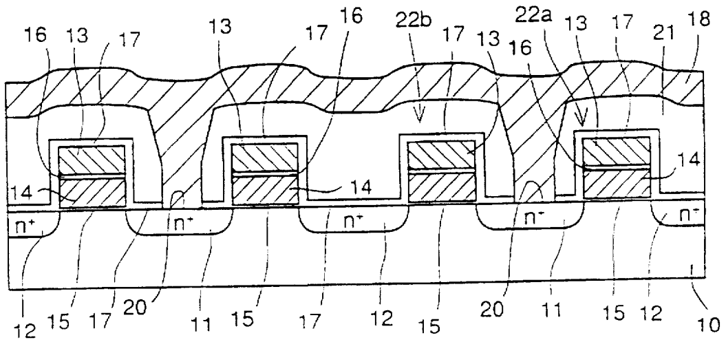
FIG. 152 PRIOR ART
