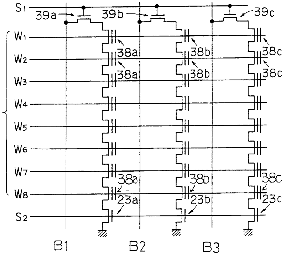
FIG. 154 PRIOR ART
