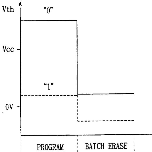
FIG. 139 PRIOR ART
