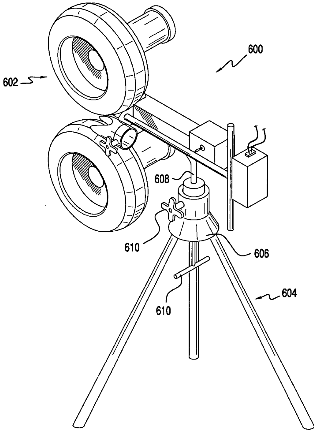
FIG. 14 (Prior Art)
