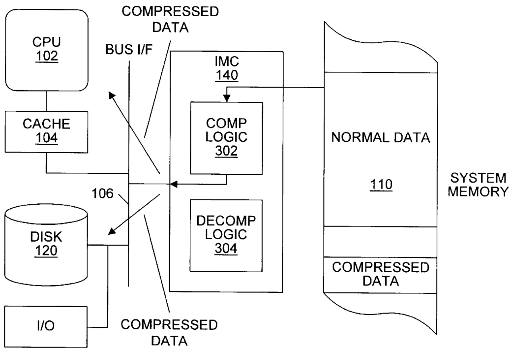
Compression from memory to CPU or Disk
