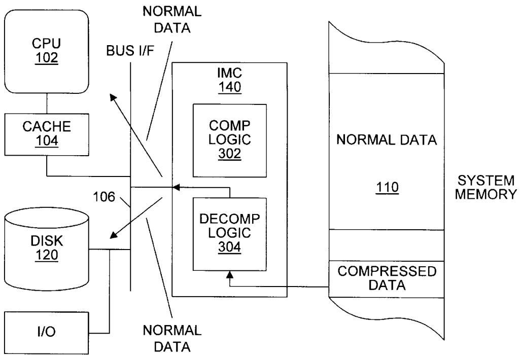
Memory decompression to CPU or Disk
