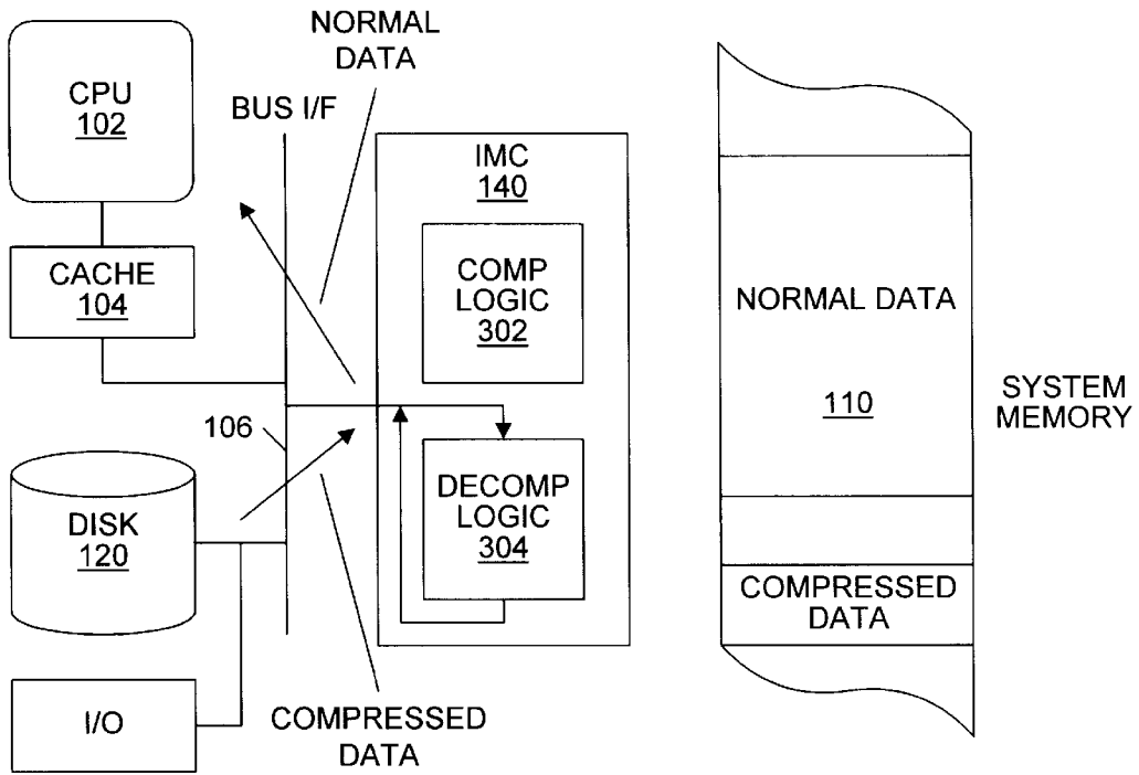
Decompression of disk to CPU
