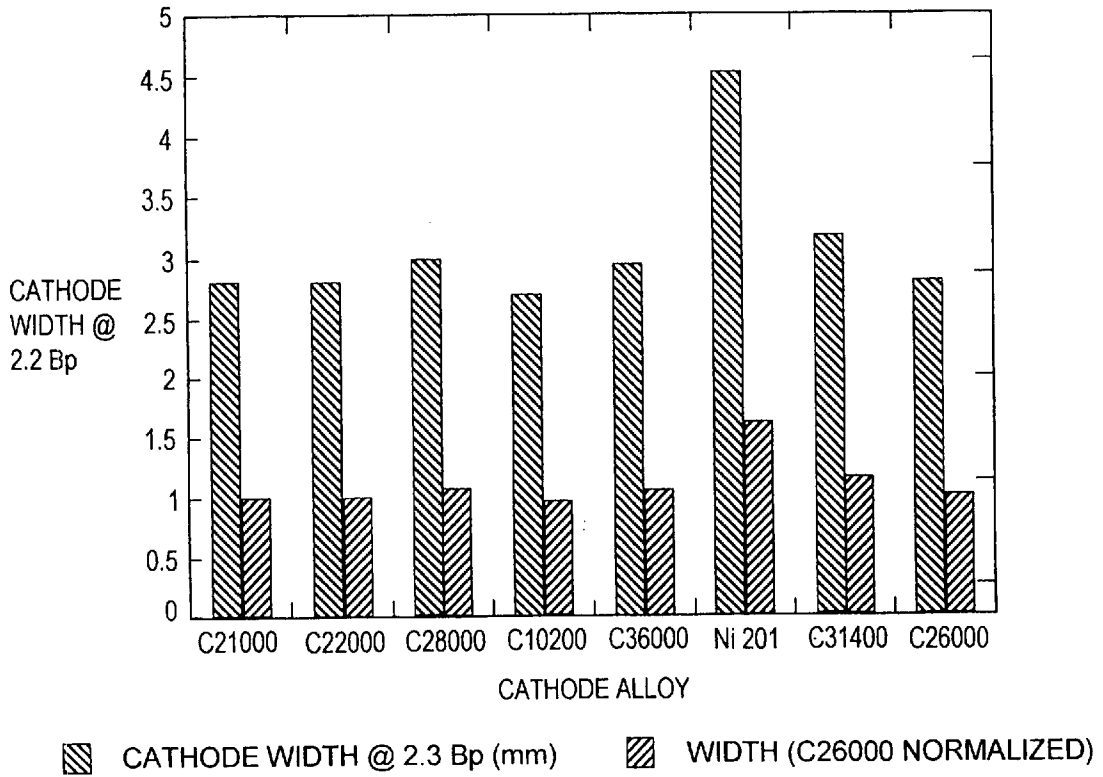
Fig. 7. Cathode Discharge Width vs Material Type (TD133, 2.5 KHz ArF, 1100 Volts, 2.3 Bp)
