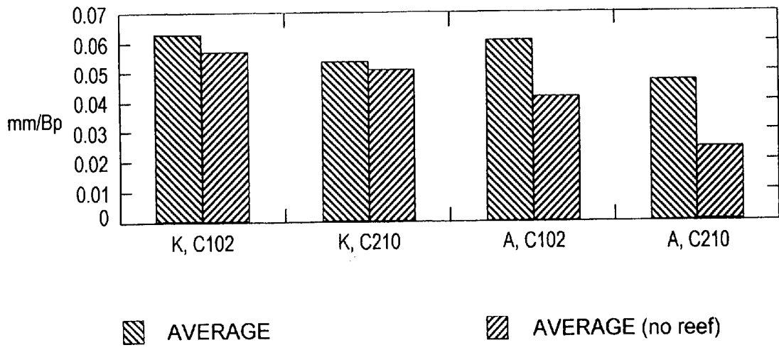
Fig. 10. Average Cathode Erosion Rates (2KHz, >2Bp)
