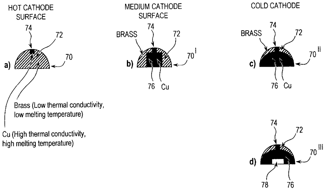
FIGURE 1. Cathode or Anode Surface Temperature Control Using Diffusion Bonding Technology.
