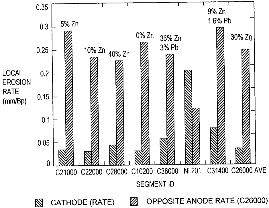
FIG. 6. LOCAL C26000 ANODE AND CATHODE SEGMENT CORROSION RATES (mm/Bp) TD133 SEGMENTED CATHODE TEST, 2.3 Bp, 2.5 KHz, ArF, 1100V
