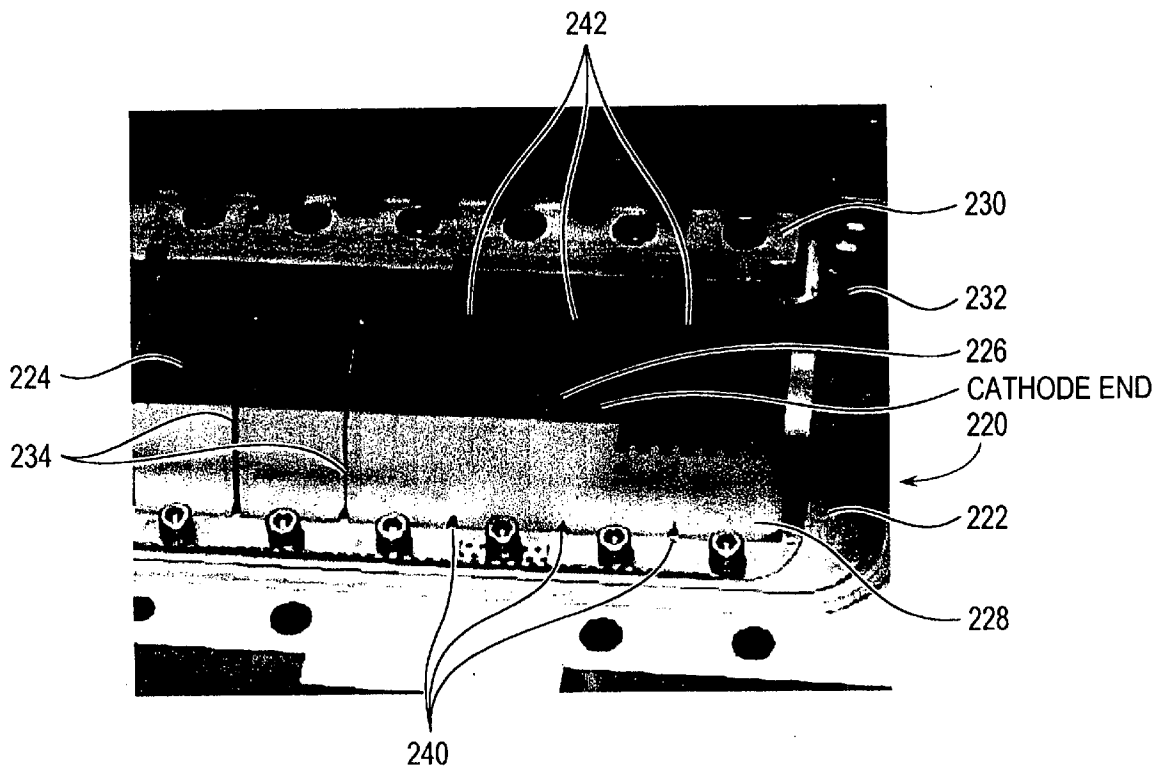
240 Current return tangs removed to increase inductance at end of discharge region.
