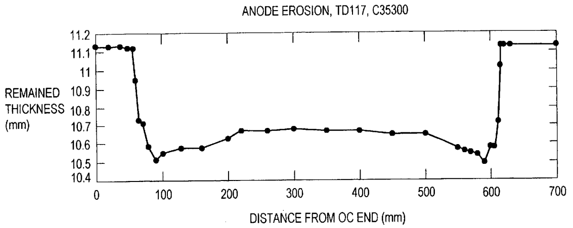
Typical Axial Anode Erosion Profile, 3 Bp in 4 KHz ArF
