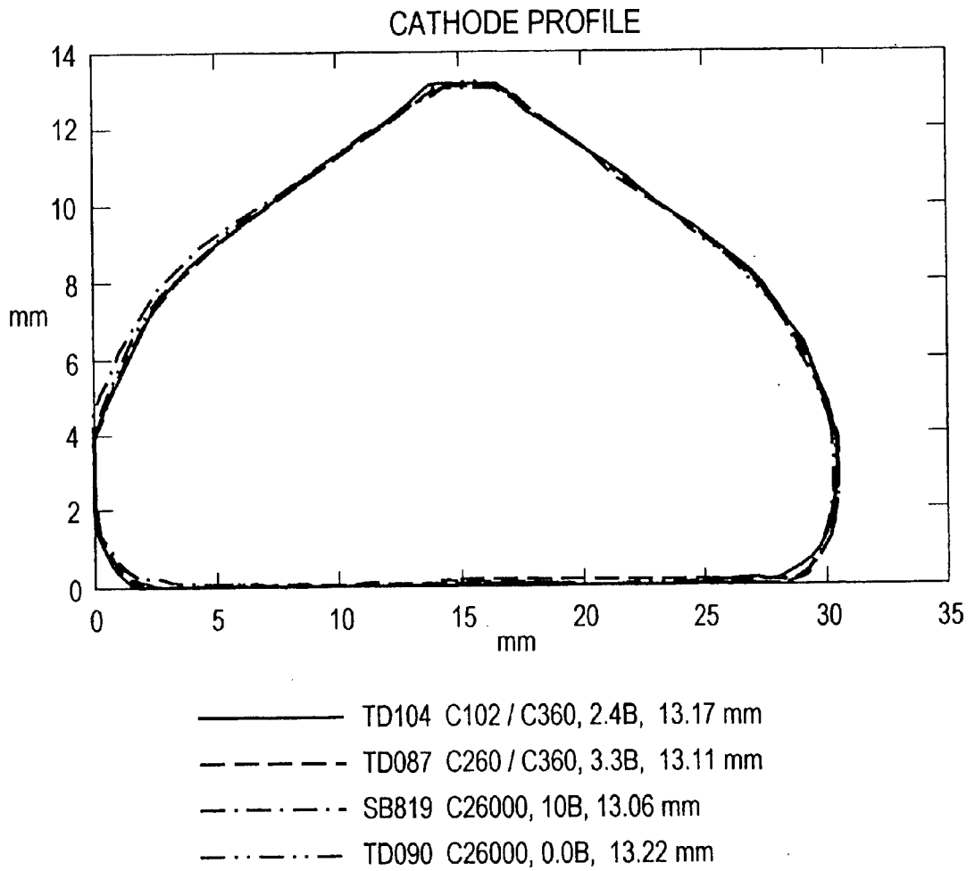
FIG. 2. Cathode Profile Changes
