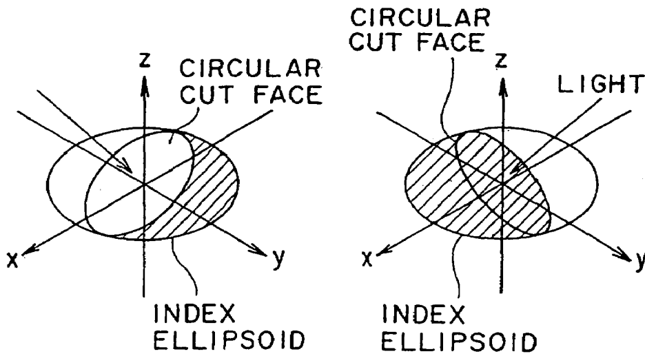
CIRCULAR CUT FACE OF INDEX ELLIPSOID
