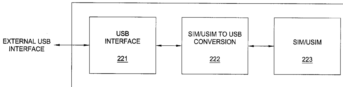
USB BASED SIM/USIM UICC DEVICE 100
