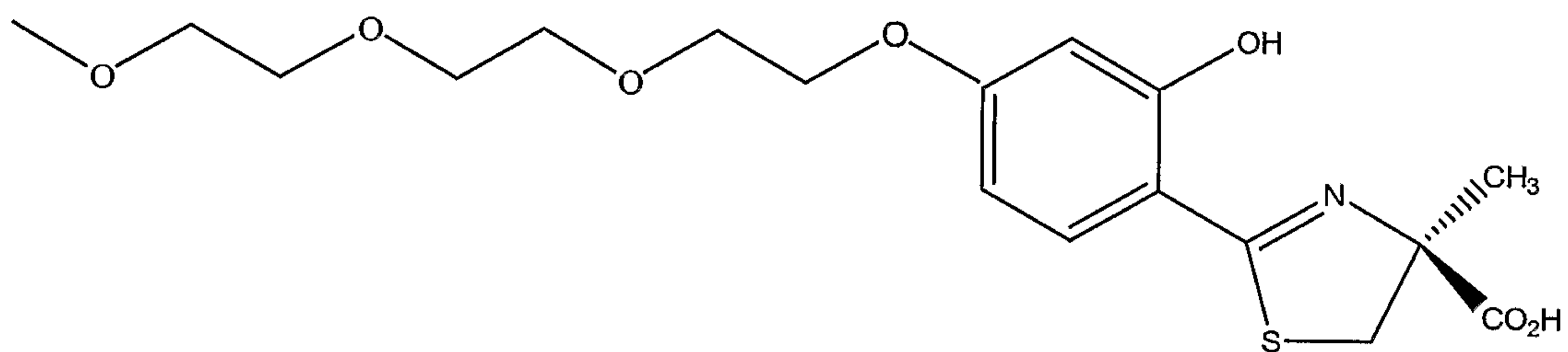
(S)-4'-(HO)-DADFT-PE
