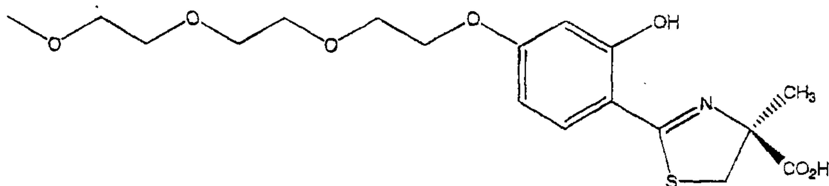
(S)-4'-(HO)-DADFT-PE
