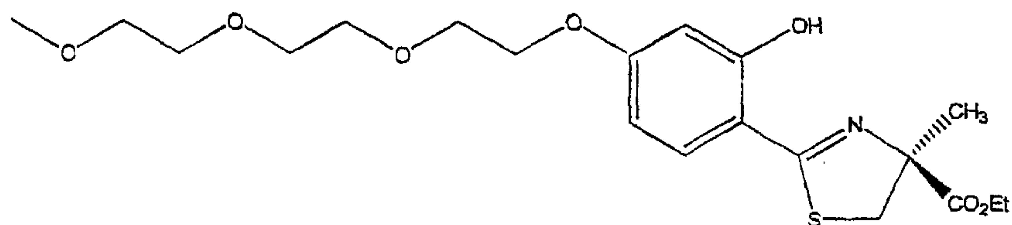
(S)-4'-(HO)-DADFT-PE-EE
