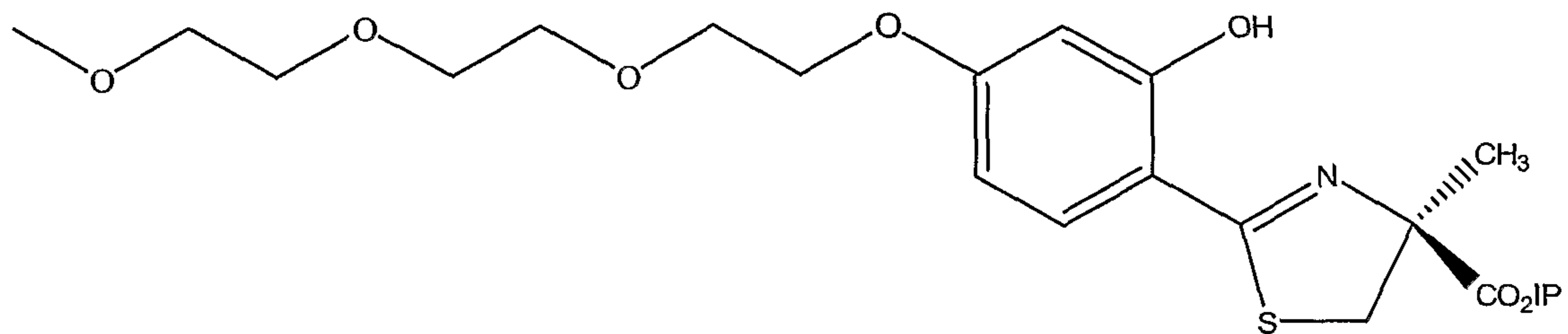
(S)-4'-(HO)-DADFT-PE iPrE
