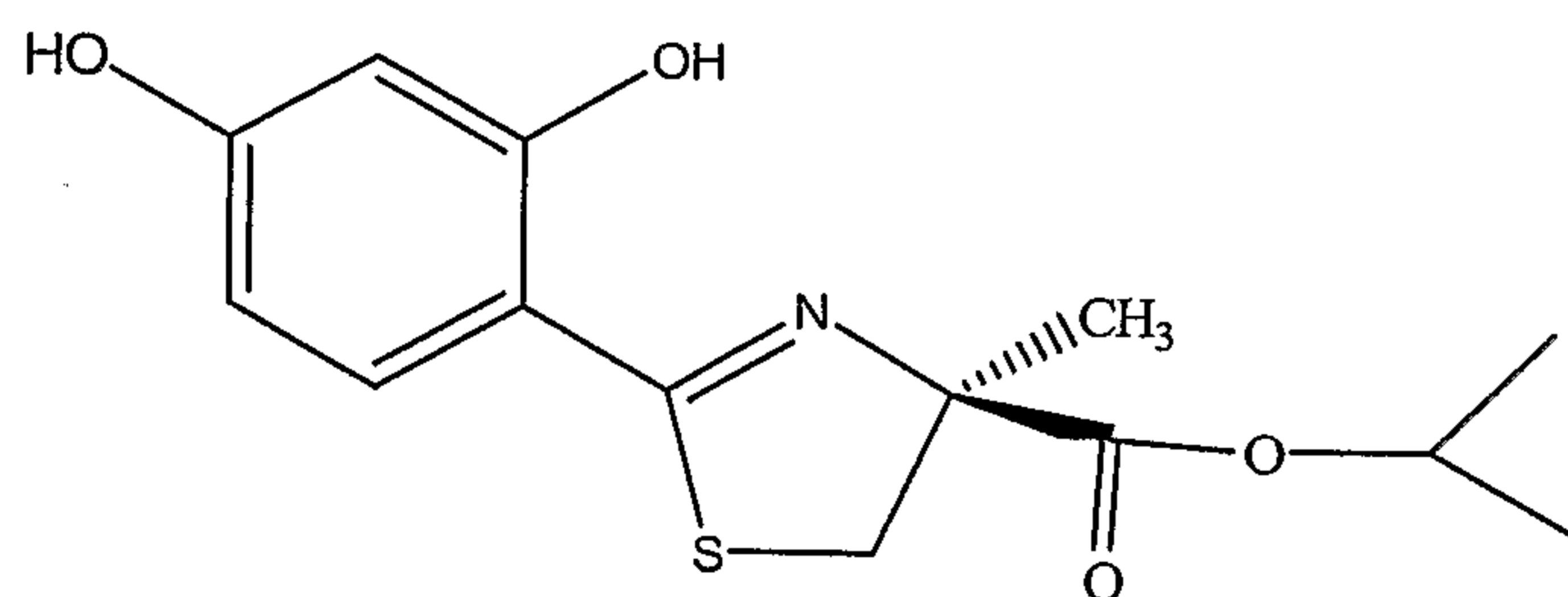
(S)-4'-(HO)-DADFT-iPrE
