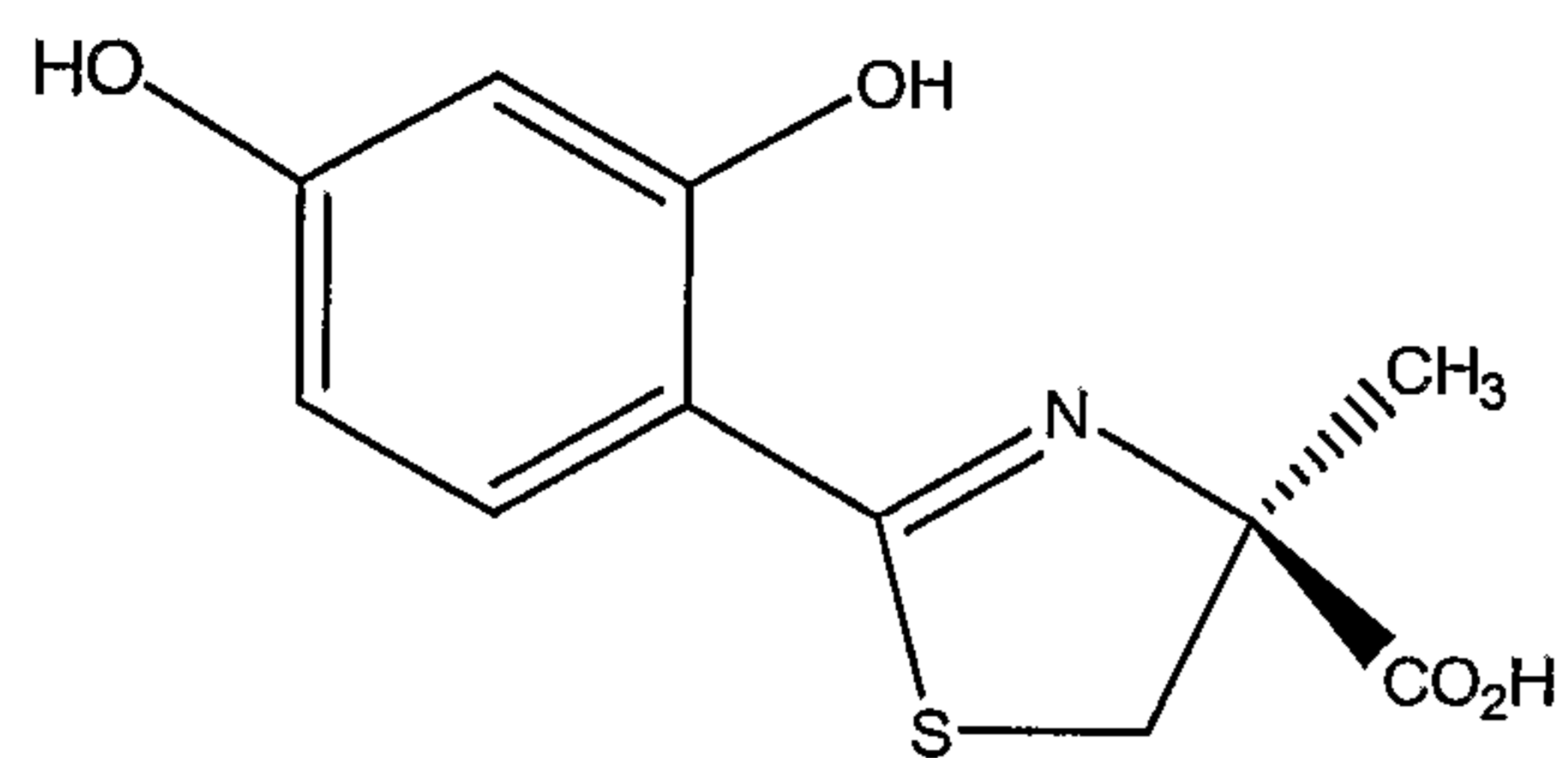
(S)-4'-(HO)-DADFT
