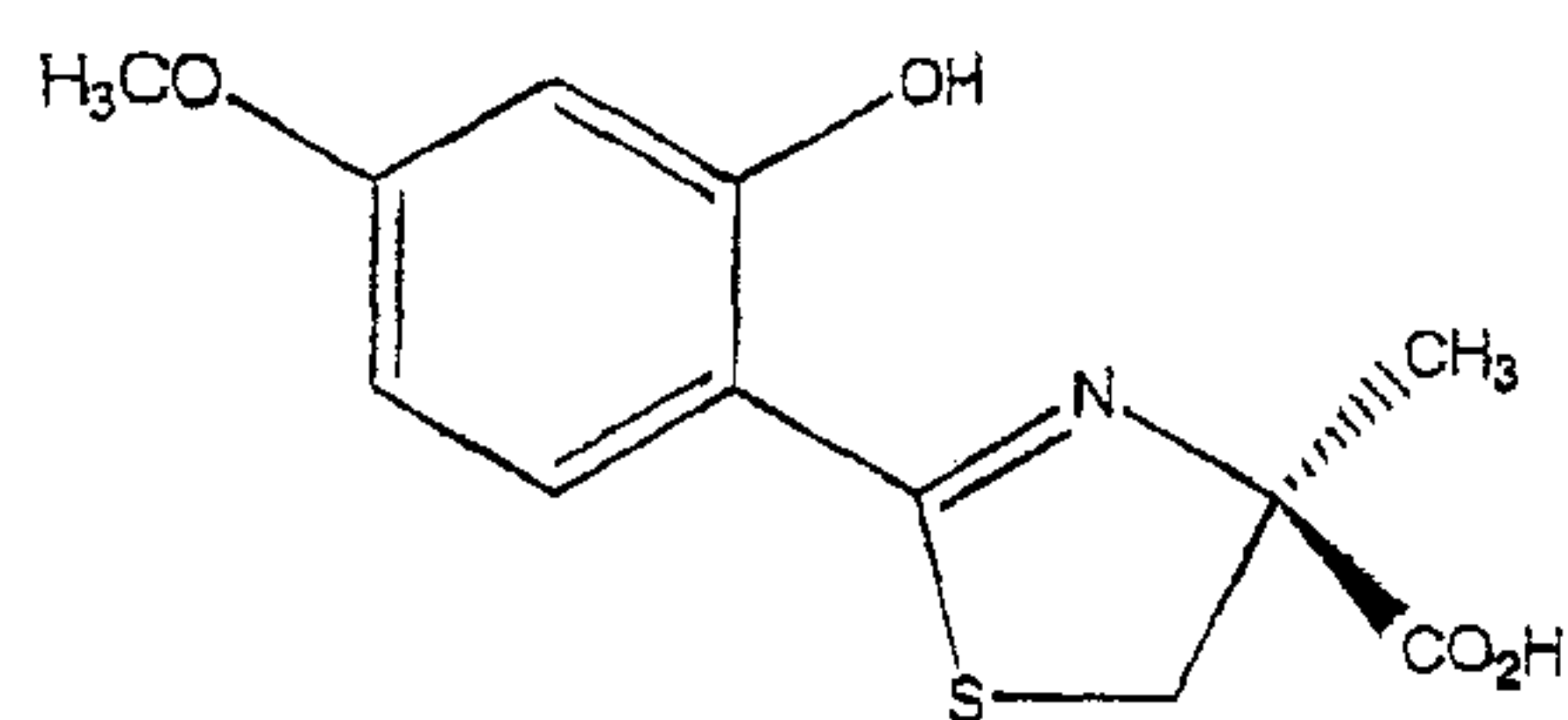
(S)-4'-(CH 3 O)-DADFT
