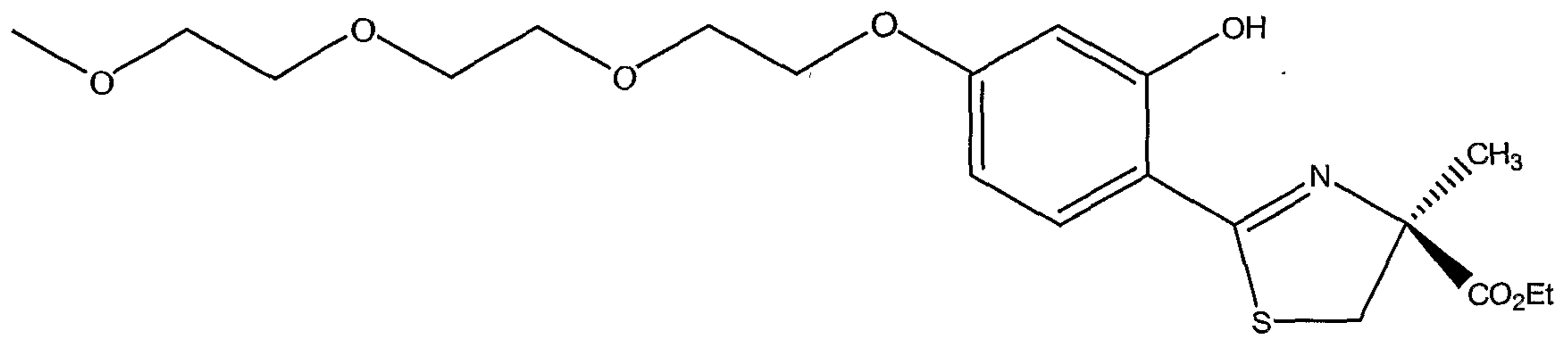
(S)-4'-(HO)-DADFT-PE EE
