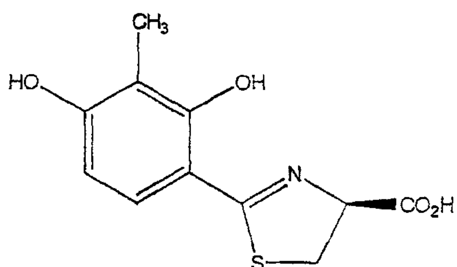
(S)-3'-(CH 3 )-4'-(HO)-DADMDFT
