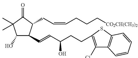
Compound 3
