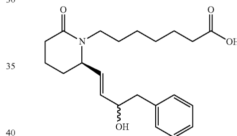
Compound 1
