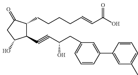
Compound 13
