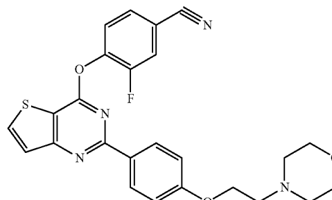
Compound 23
