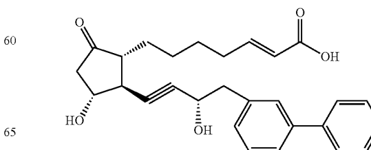
Compound 11
