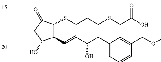
Compound 7
