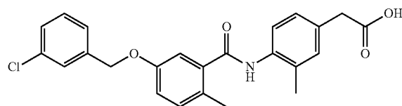
Compound 24
