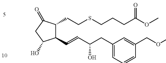
Compound 6
