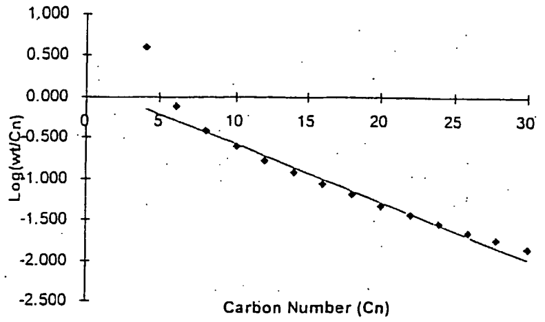
Figure 1: Regression Analysis of Example 2
