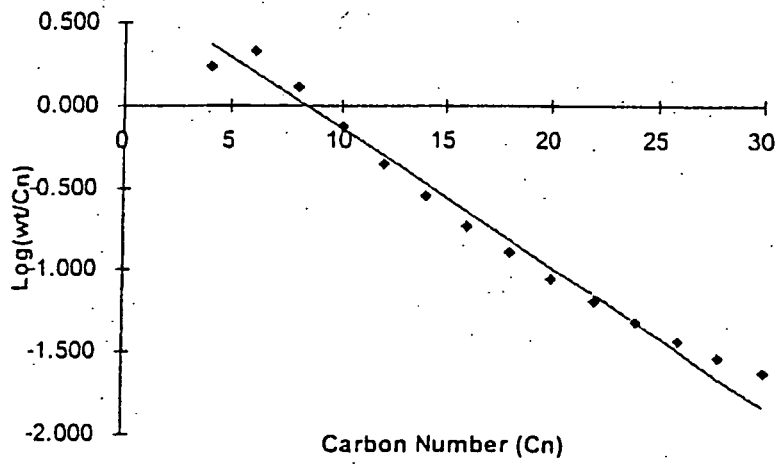
Figure 2: Regression Analysis of Example 5
