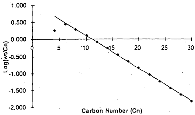
Figure 4: Regression Analysis of Example 10
