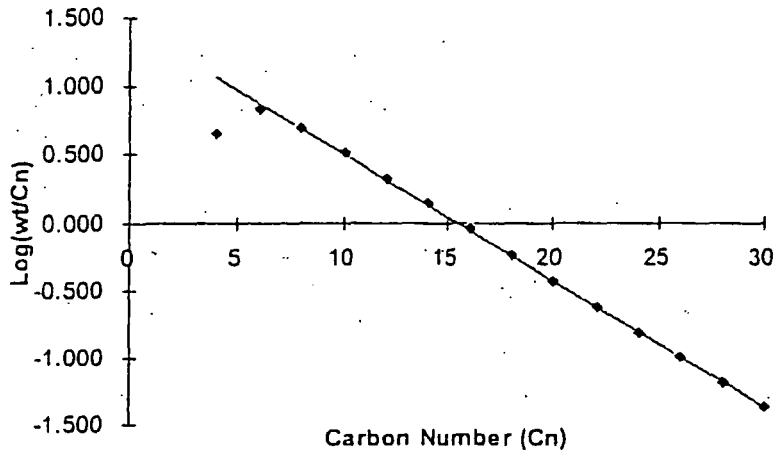
Figure 3: Regression Analysis of Example 8
