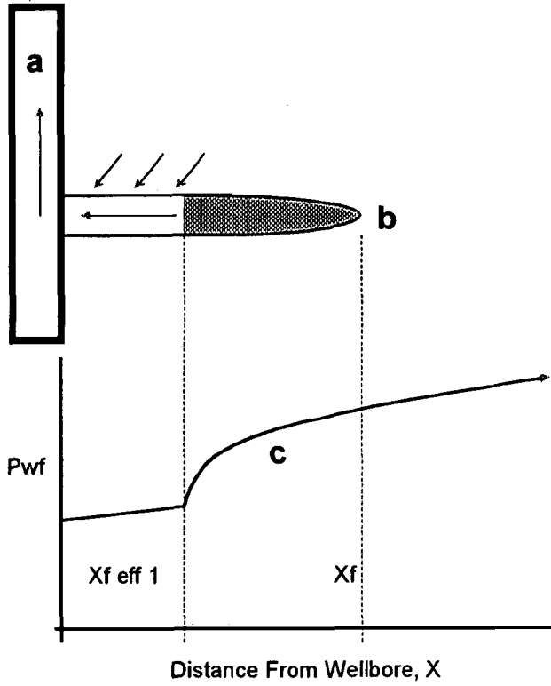
Figure 1A: Fracture-Stimulated Gas Well Before Process
