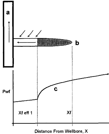
Fracture-Stimulated Gas Well Before Process
