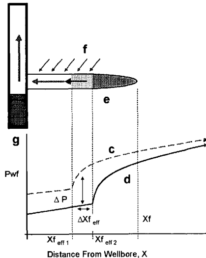
Well After Process
