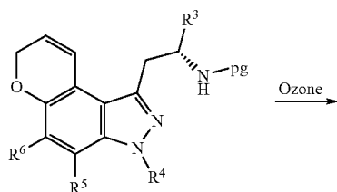
Scheme 3
