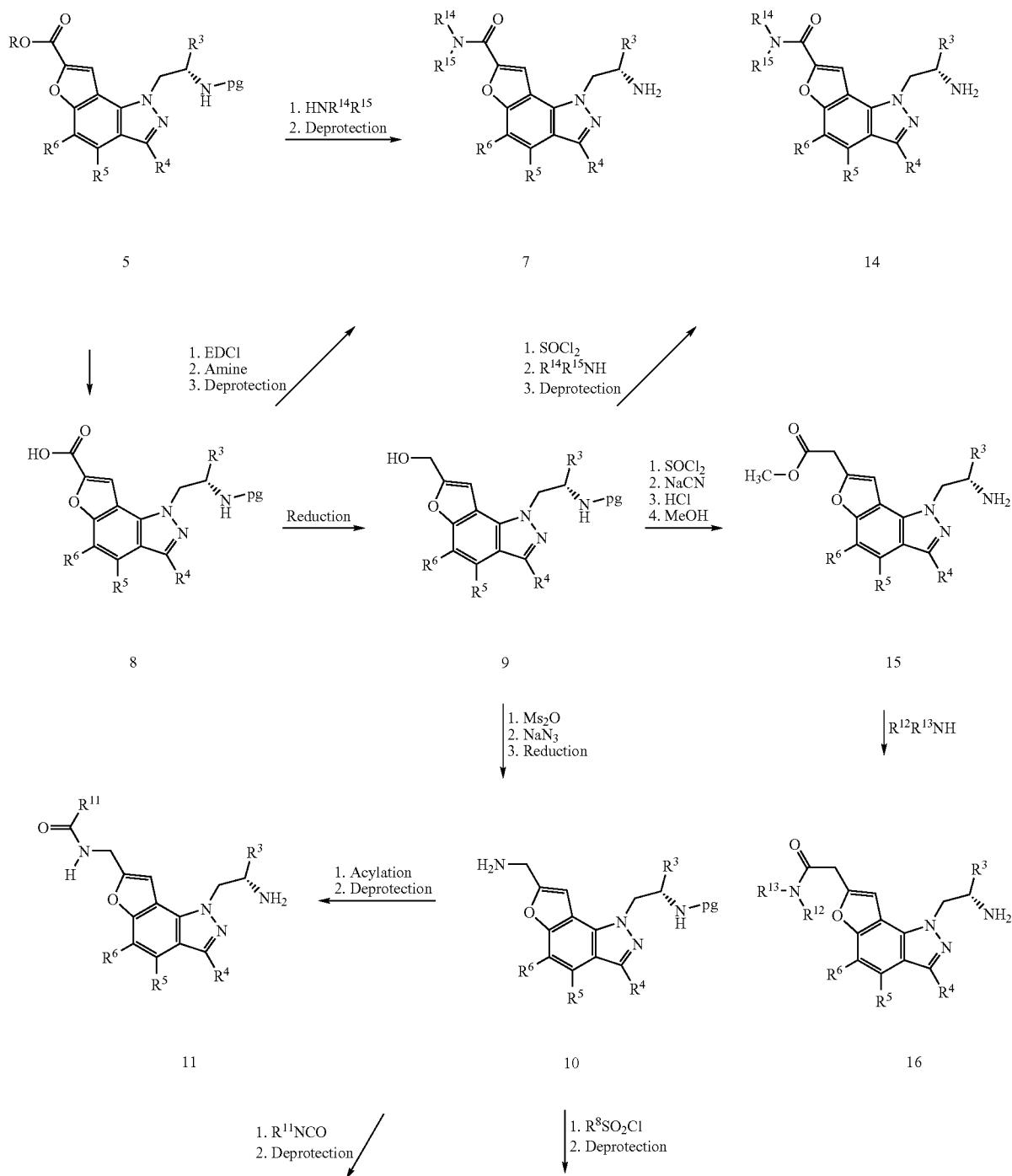
Scheme 2:
