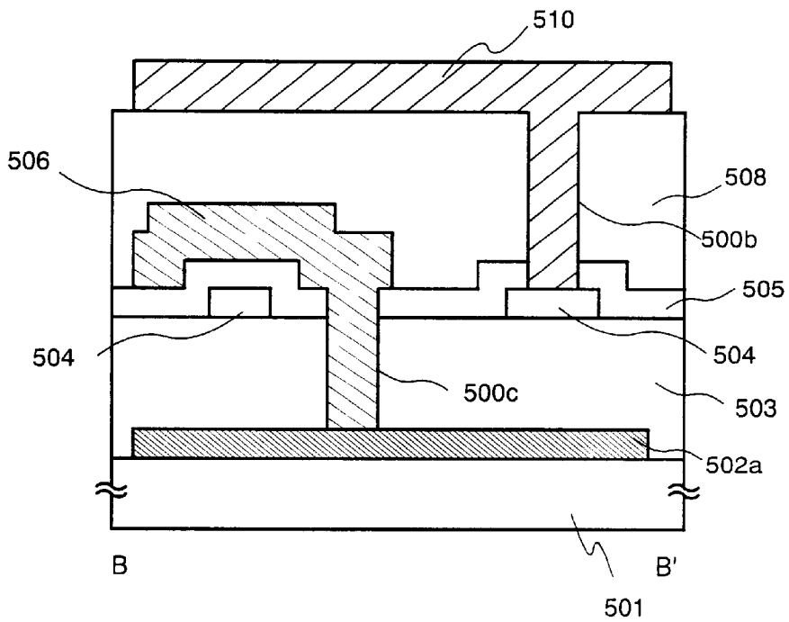
Fig. 15B B-B' Cross sectional view
