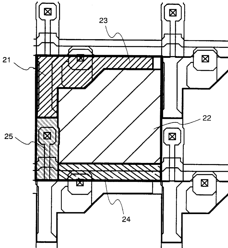
Fig. 19 Prior Art
