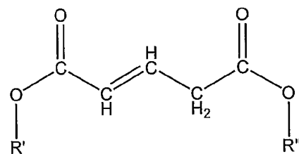
Monoester of 2-Pentenedioic Acid
