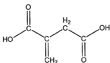
Itaconic Acid
