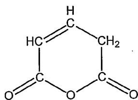
2-Pentendioic Anhydride
