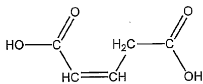
2-Pentendioic Acid
