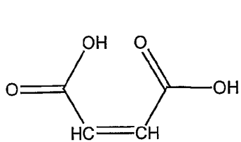
Maleic Acid
