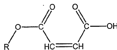
Monoester of Maleic Acid
