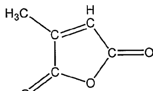
Citraconic Anhydride
