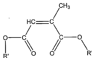
Monester of Citraconic Acid
