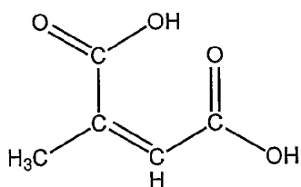
Citraconic Acid
