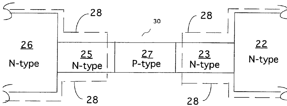
Figure 1B (Prior Art)
