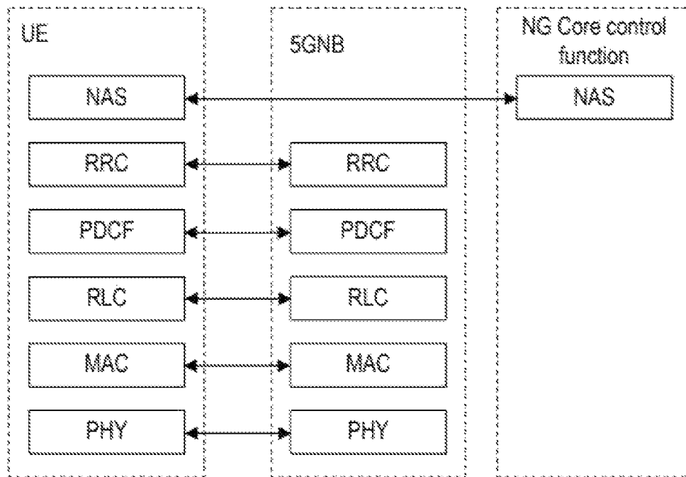
Control Plane Protocol Stack
