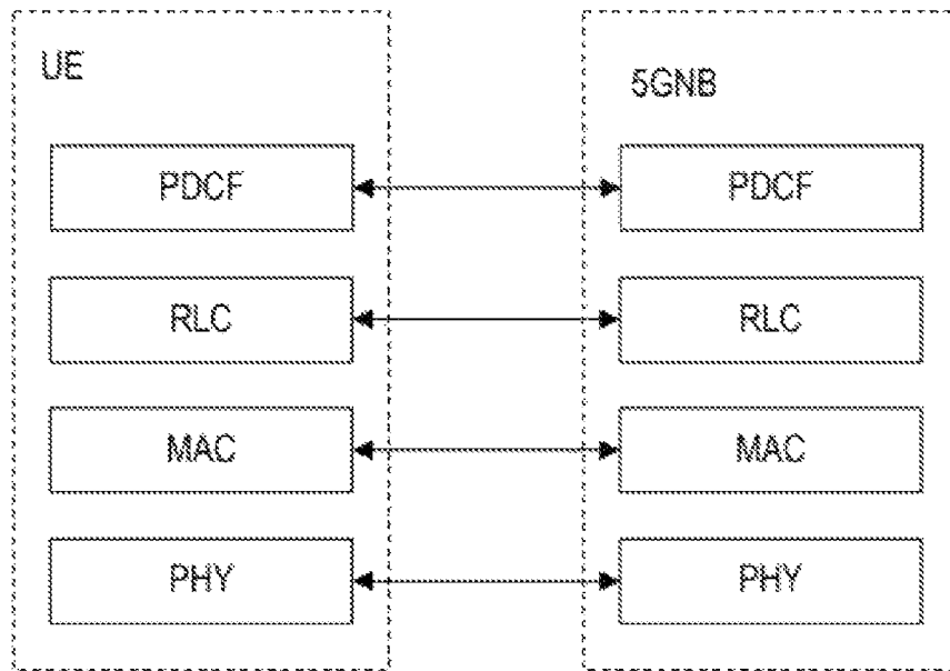
User Plane Protocol Stack
