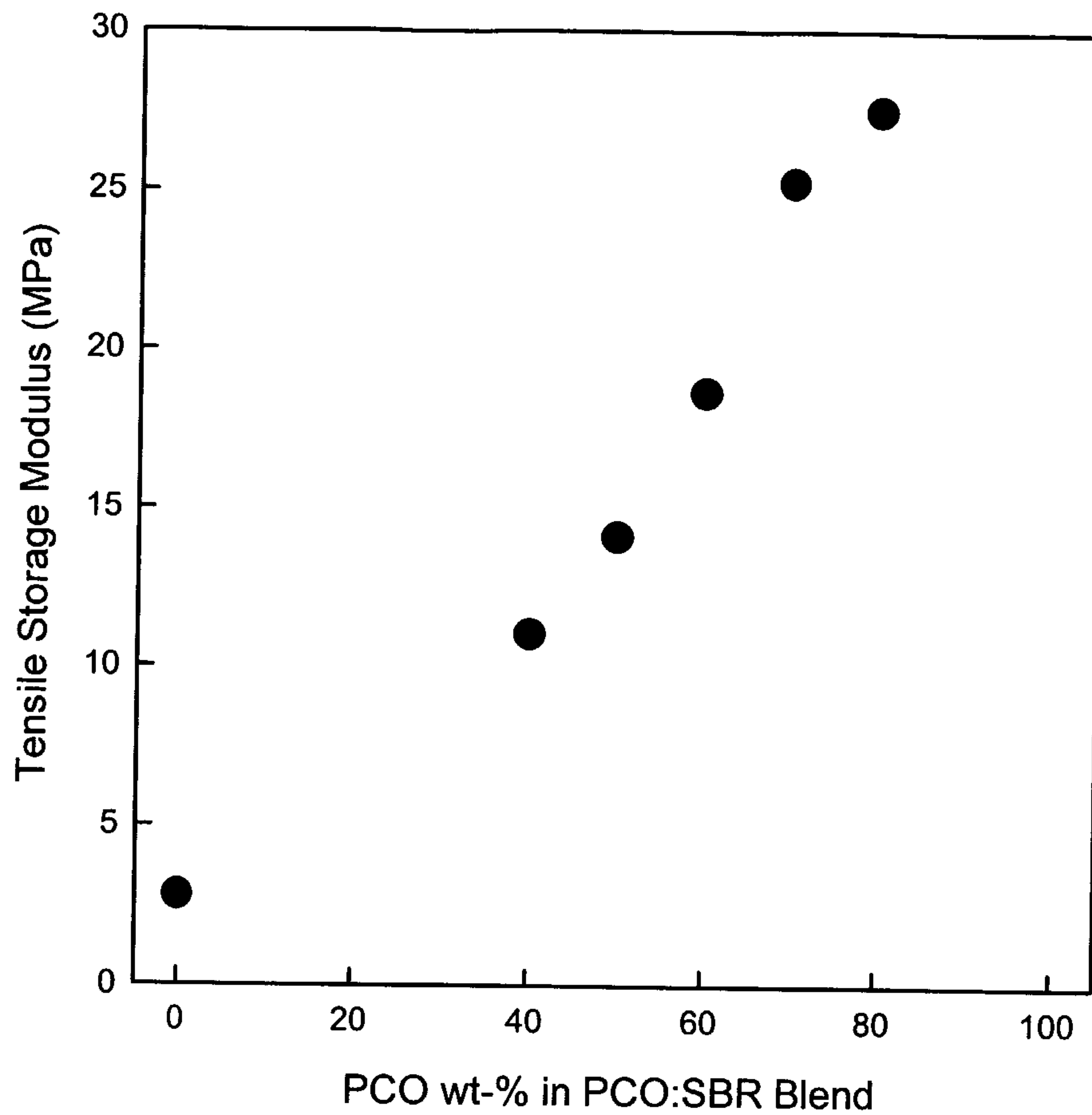
Figure 7. Dependence of tensile storage modulus on PCO wt-% in PCO:SBR blends prepared by melt blending and crosslinking with 1 wt-% PCO at T = 180 °C for 30 min.
