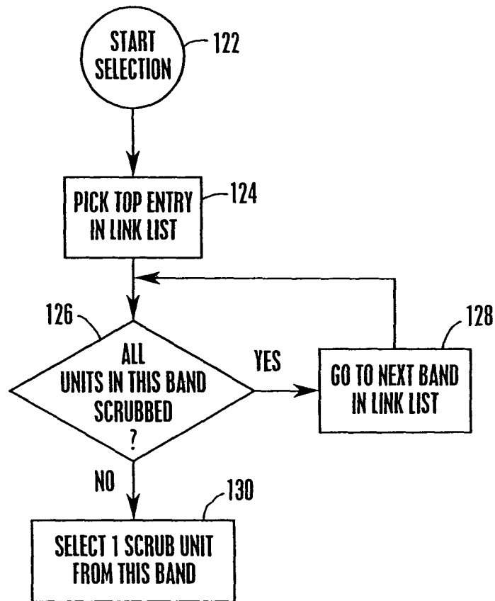
Fig. 10 Divide The Disk Into Bands - Selection Algorithm
