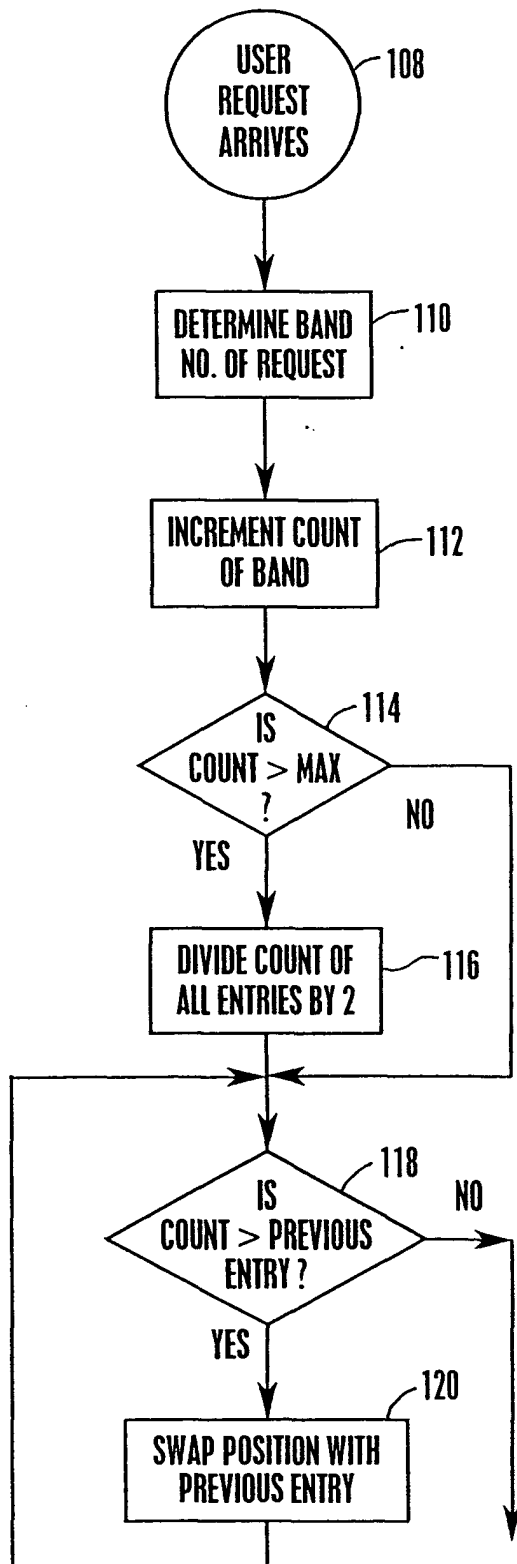
Fig. 9 Divide The Disk Into Bands - Table Maintenance
