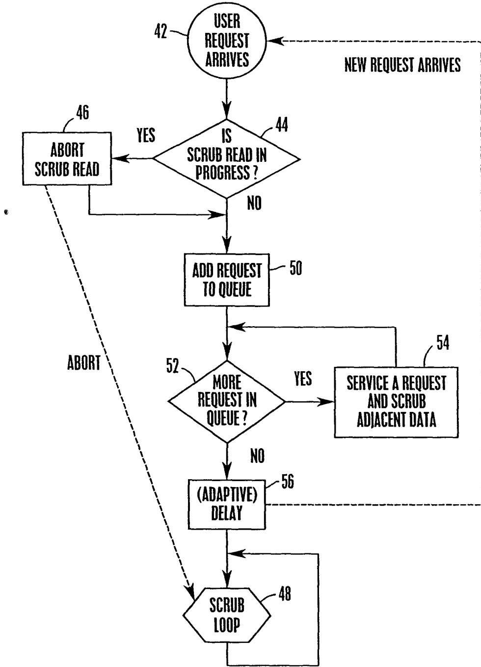
Fig. 4 Interrupt of Scrub with Delay, opportunistic options
