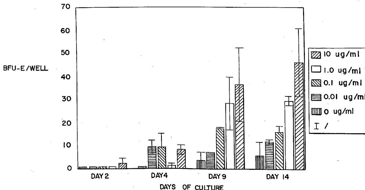
EFFECT OF IGD ON FORMATION OF HUMAN BURST FORMING UNITS-ERYTHROID
