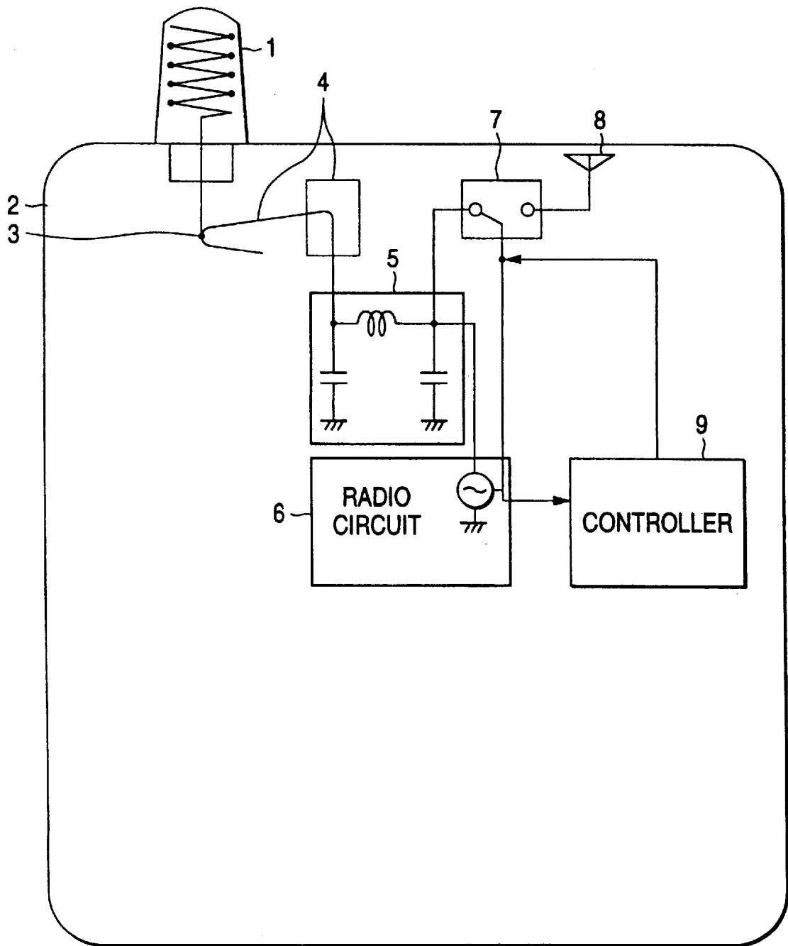
FIG. 4 PRIOR ART
