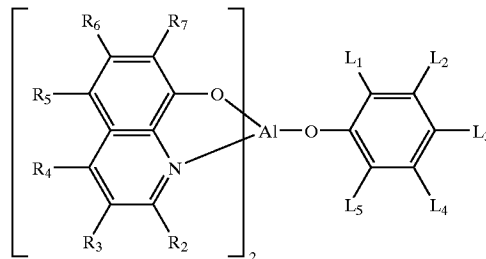
[Chem 4]
