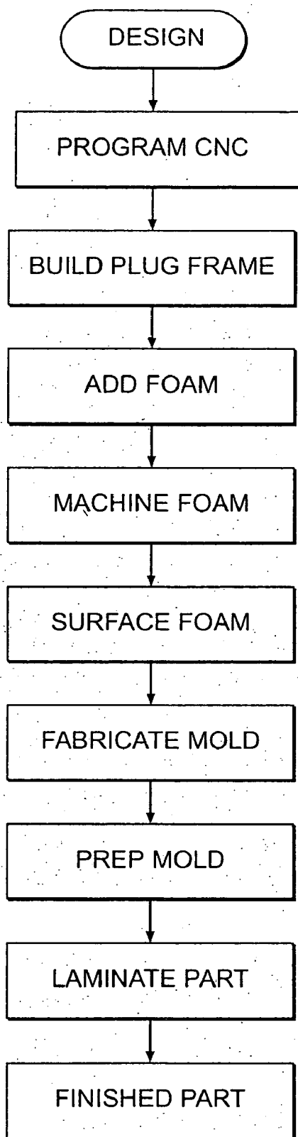
FIG. 4 PRIOR ART
