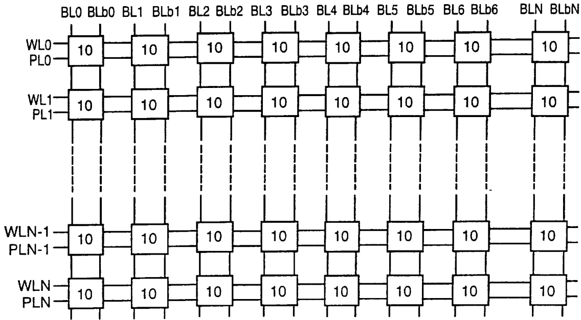
Fig. 4 Prior Art
