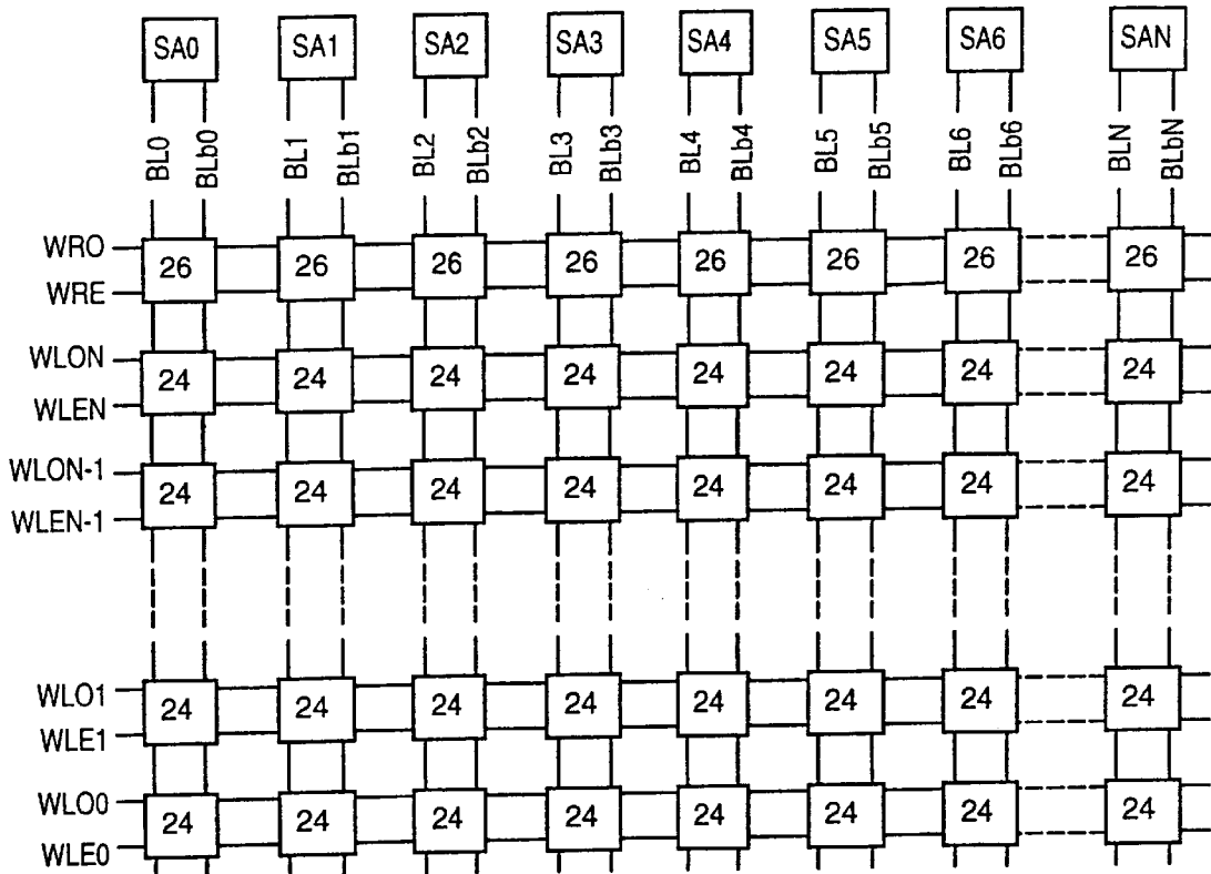
Fig. 9 Prior Art
