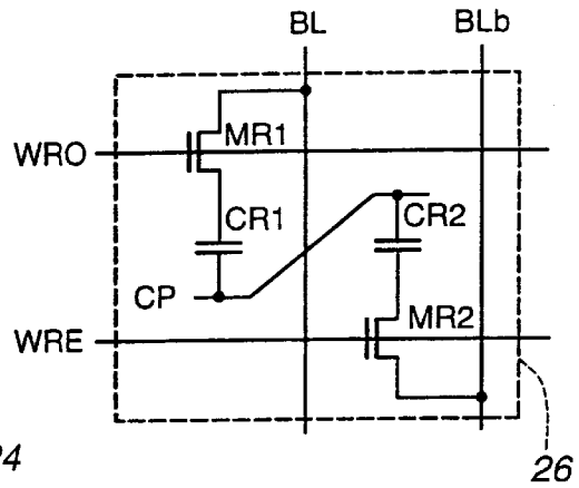
Fig. 8 Prior Art
