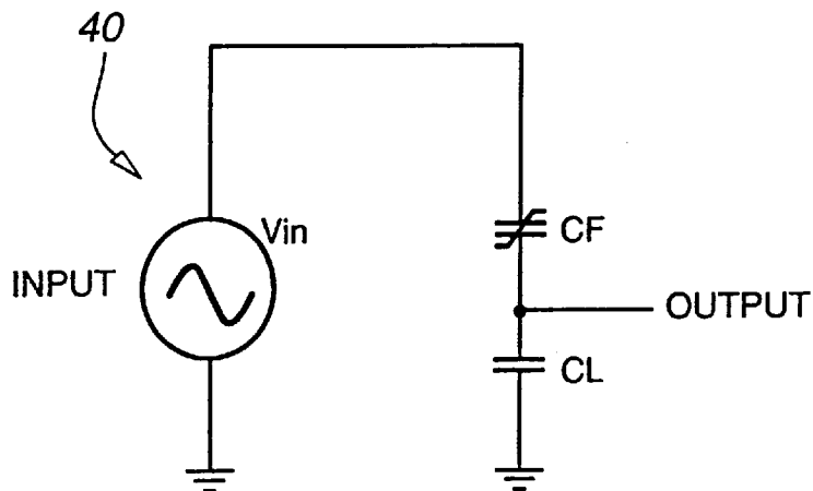
Fig. 11 Prior Art
