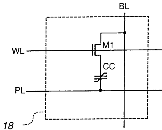
Fig. 2 Prior Art
