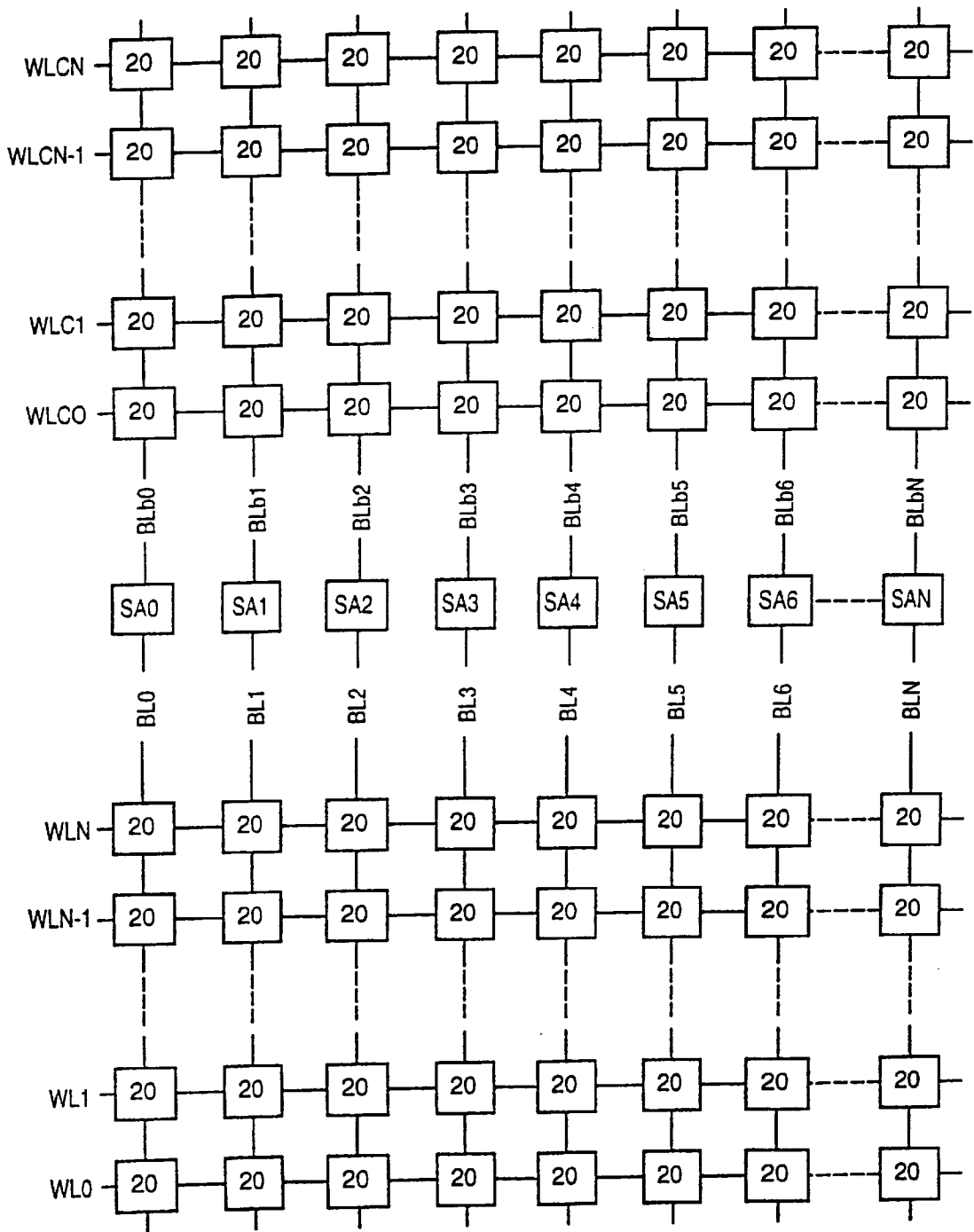
Fig. 6 Prior Art
