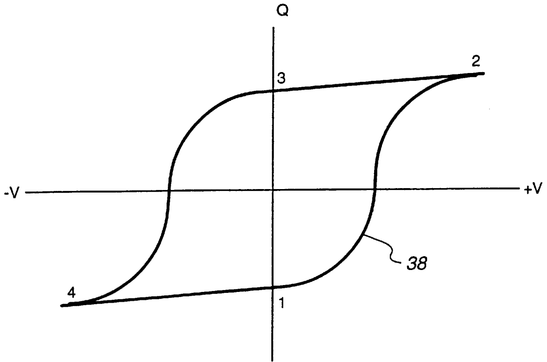
Fig. 10 Prior Art
