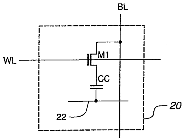
Fig. 5 Prior Art
