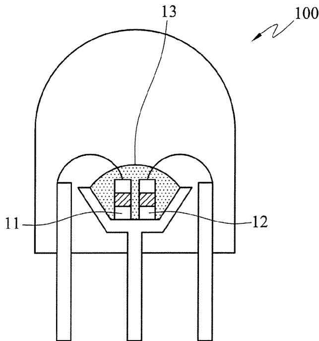
FIG. 2 (PRIOR ART)
