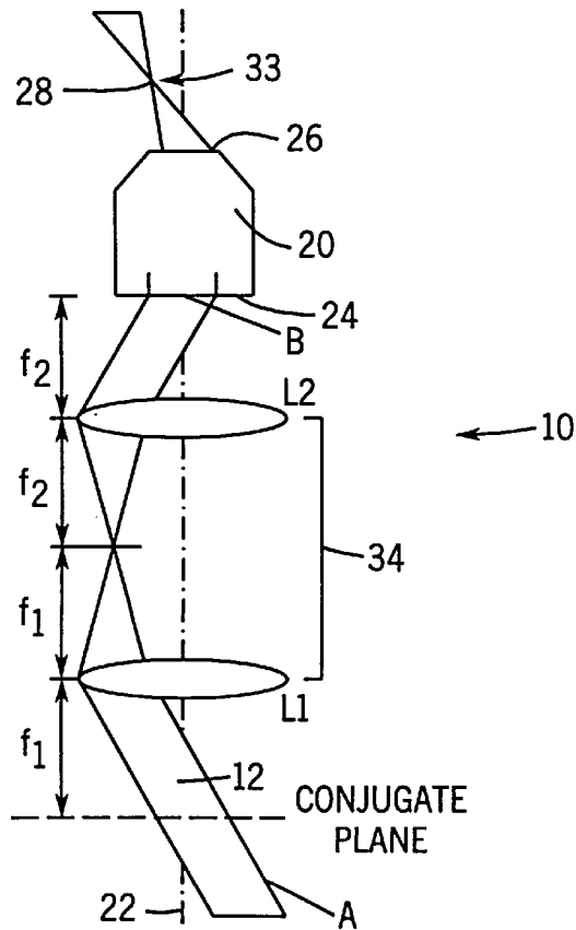
FIG. 2 PRIOR ART
