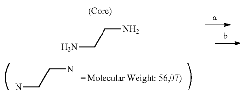
Scheme 1. Synthesis of a PAMAM-GO dendrimer.
