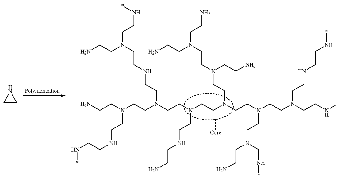
Scheme 2. Synthesis of a PEI hyperbranched polymer.
