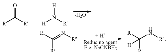
Scheme 4. Reductive amination
