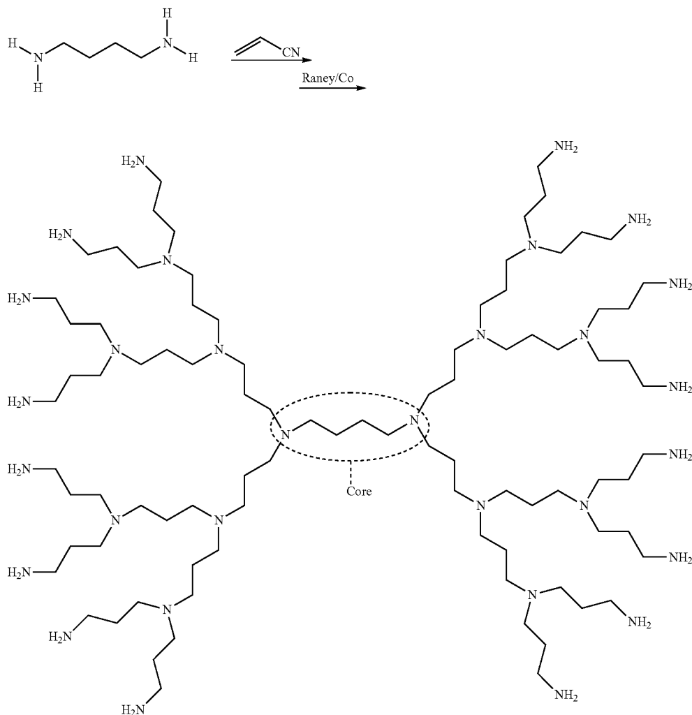
Scheme 3. Synthesis of PPI dendrimer.
