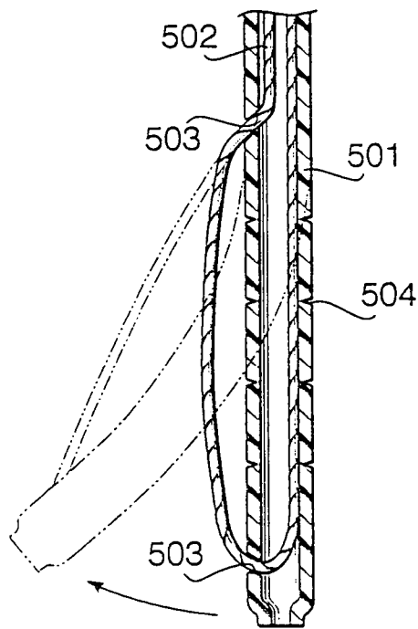
FIG. 35 PRIOR ART
