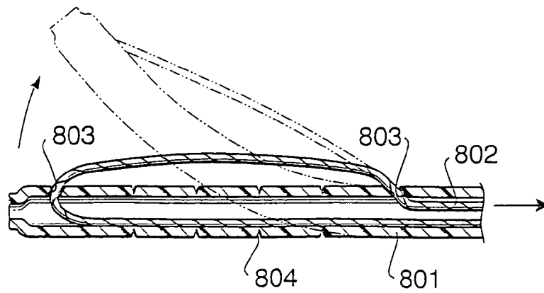
FIG. 52 PRIOR ART
