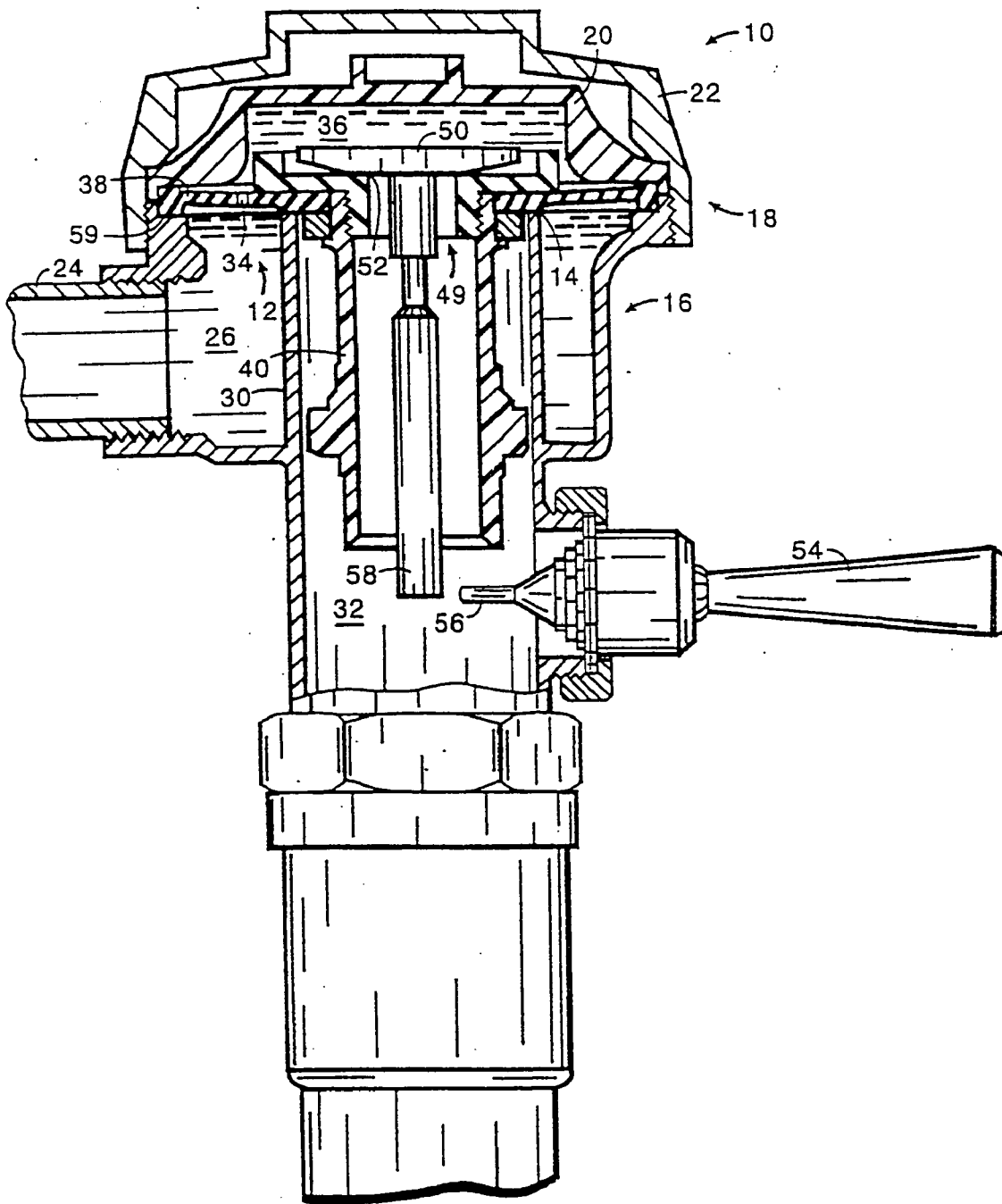
FIG. 1 (PRIOR ART)
