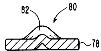
FIG. 6C (PRIOR ART)
