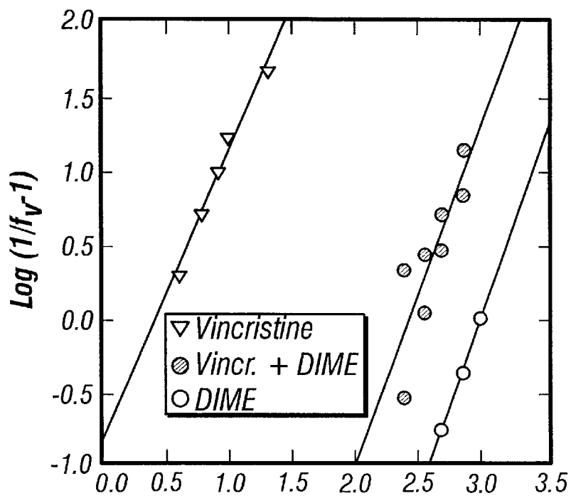
\text{Log}(I_1 + I_2)
