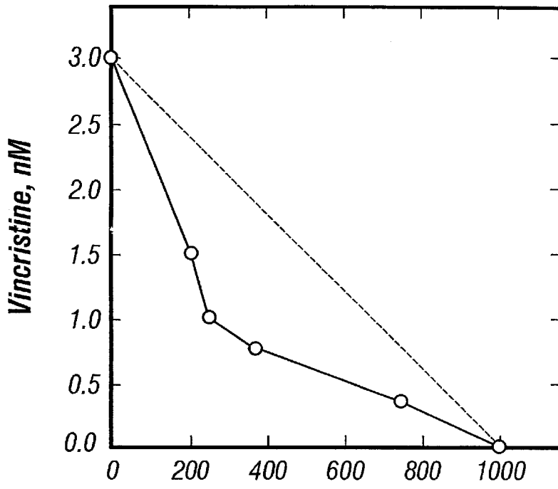
DIME, nM
