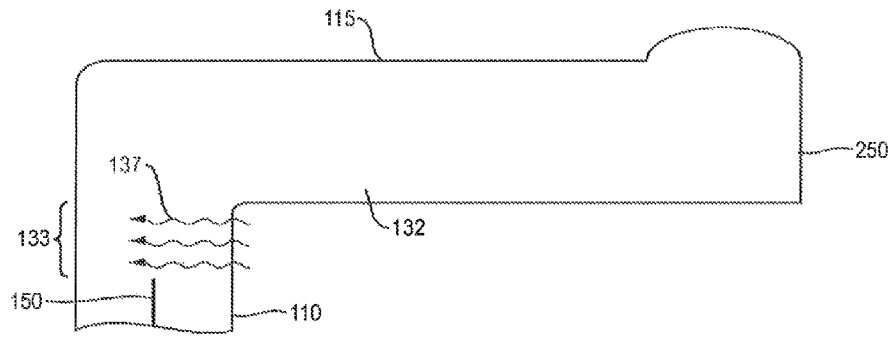
FIG. 12 (PRIOR ART)
